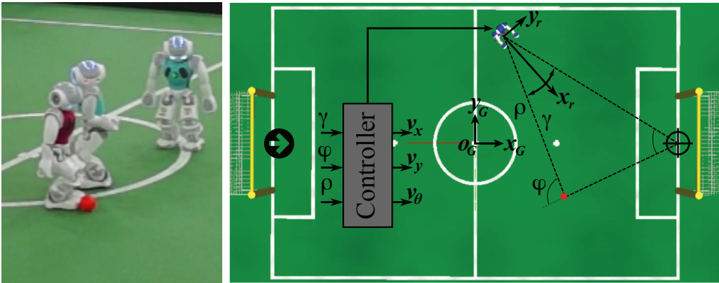
Figure 7: A picture of the NAO robot dribbling during a RoboCup SPL game (left), and definition of variables for dribbling modeling (right).
