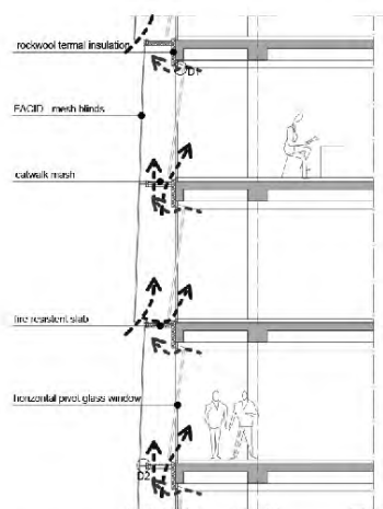
SECTION PLANE, SEGMENT OF FACADE
