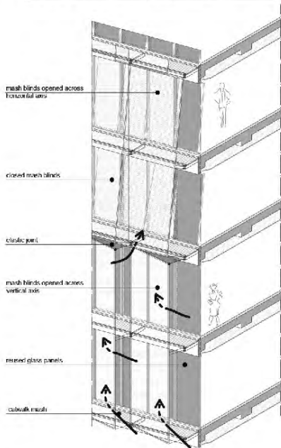
ISOMETRIC VIEW, SEGMENT OF FACADE
