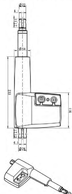
Technical detail of linear actuator
