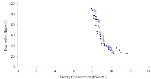
Legend: Light blue cloud dots: possible combinations of January and July Pareto front. Blue dots: Adaptive facades - better combinations of January and July Pareto front. Black dots: Static facade.
