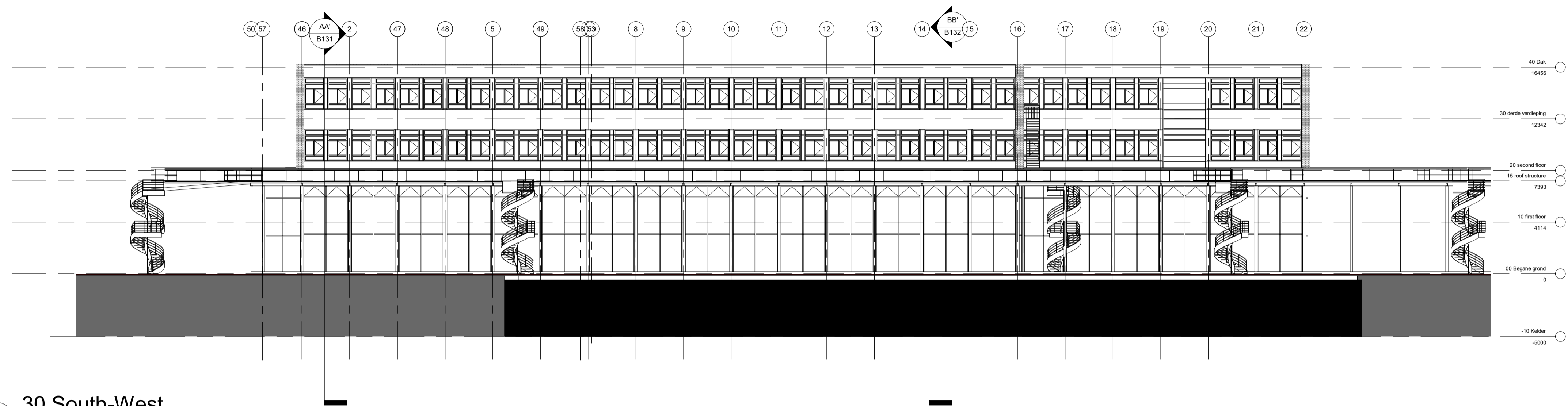
1 30 South-West 1 : 200
