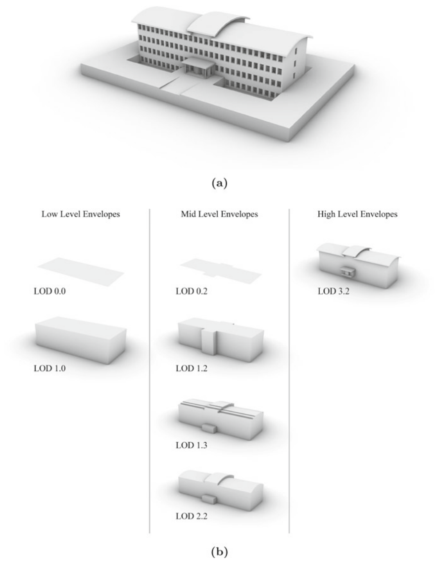
Fig. 4 The possible extracted shells of the IFC_BuildingEnvExtractor are categorised in three different levels of quality. Low level shells are accurately created from any quality model. Mid level shells are only accurately created from models that have well defined roofing structures. High level shells are only created from models that have well defined objects that construct the outer shell. All shells are generated from the model in Fig. 4a
