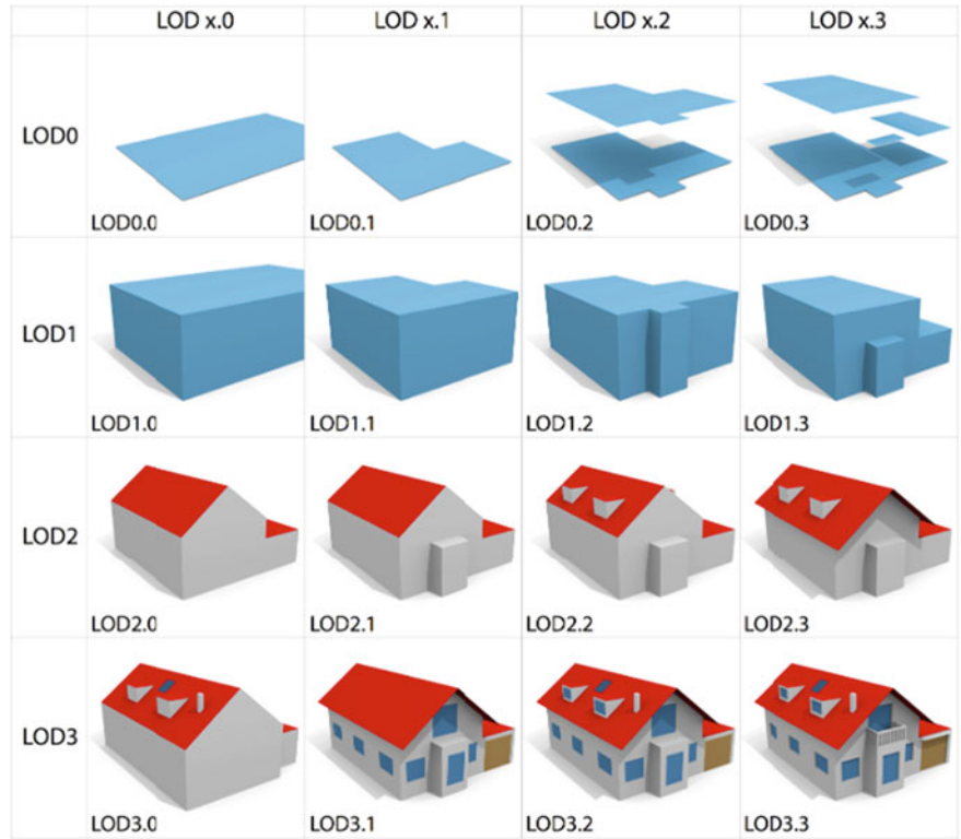
Fig. 3 The refined LoD specification of Biljecki et al. (2016)
