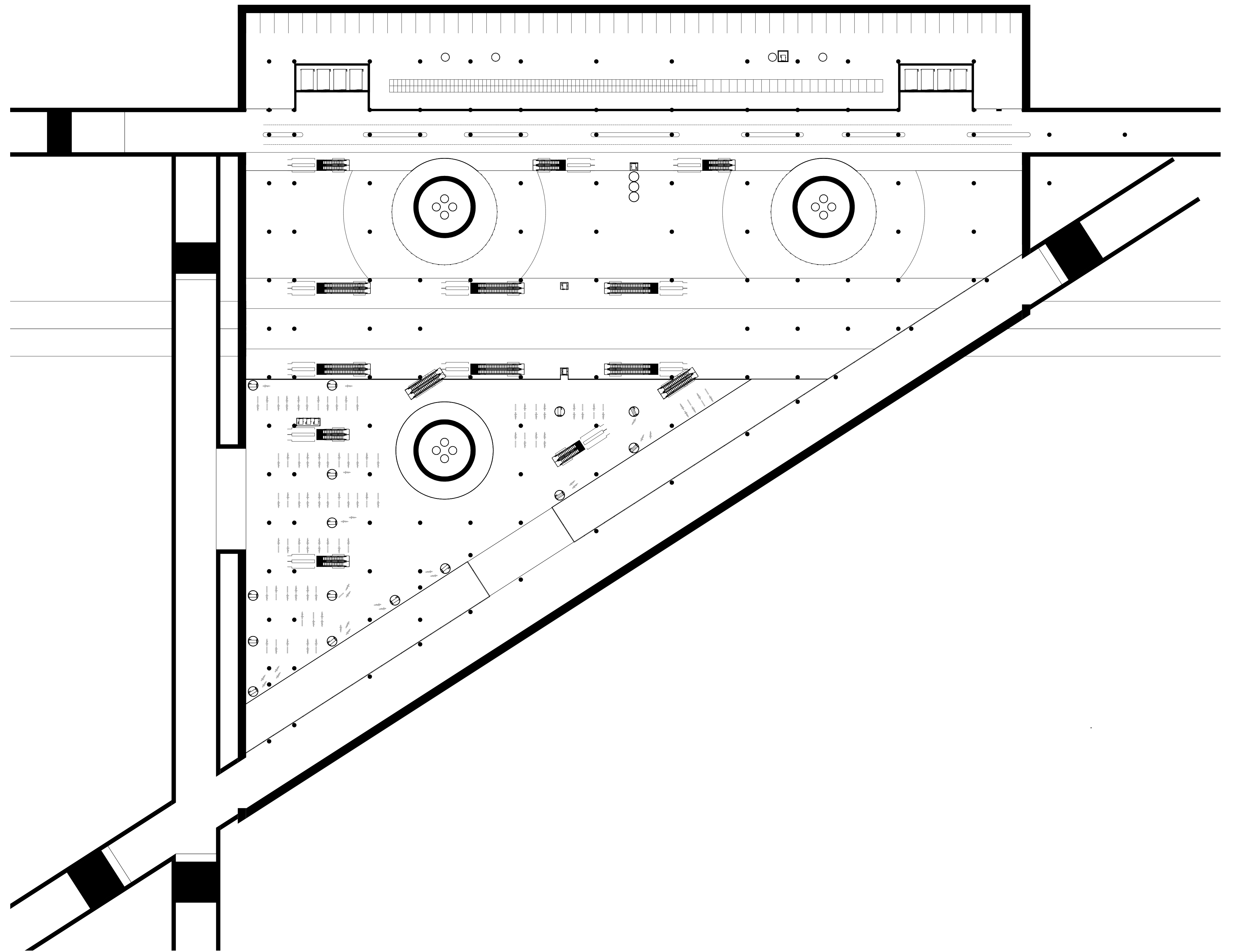
Plan - Level -1 | 1:500
