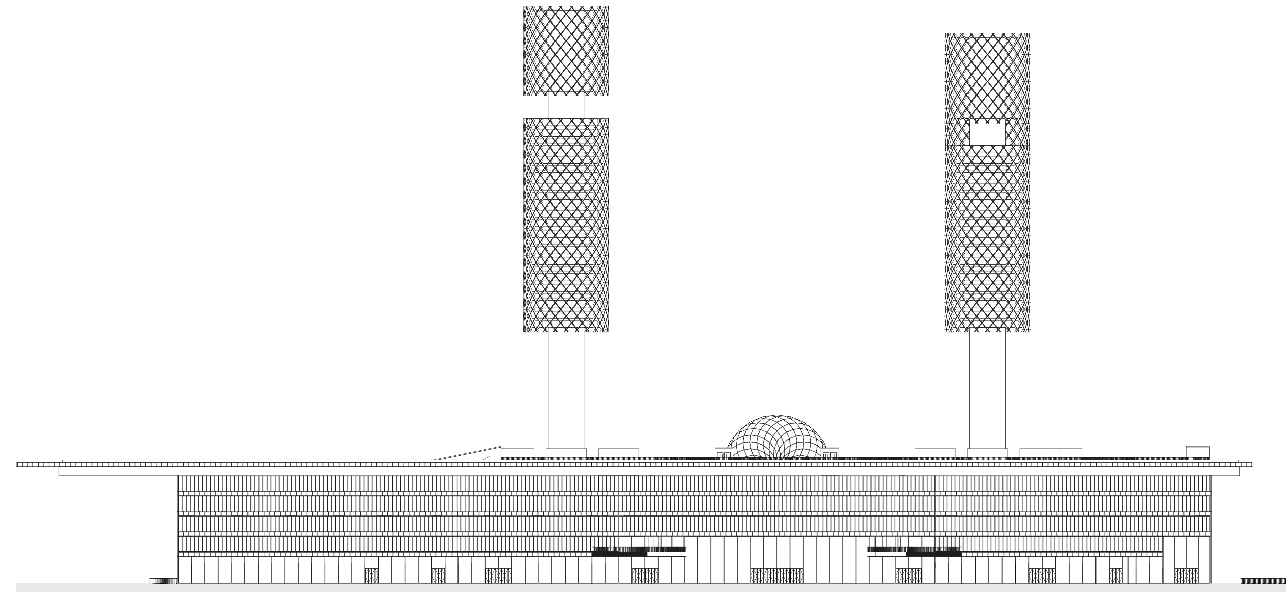
Elevation - North | 1:500
