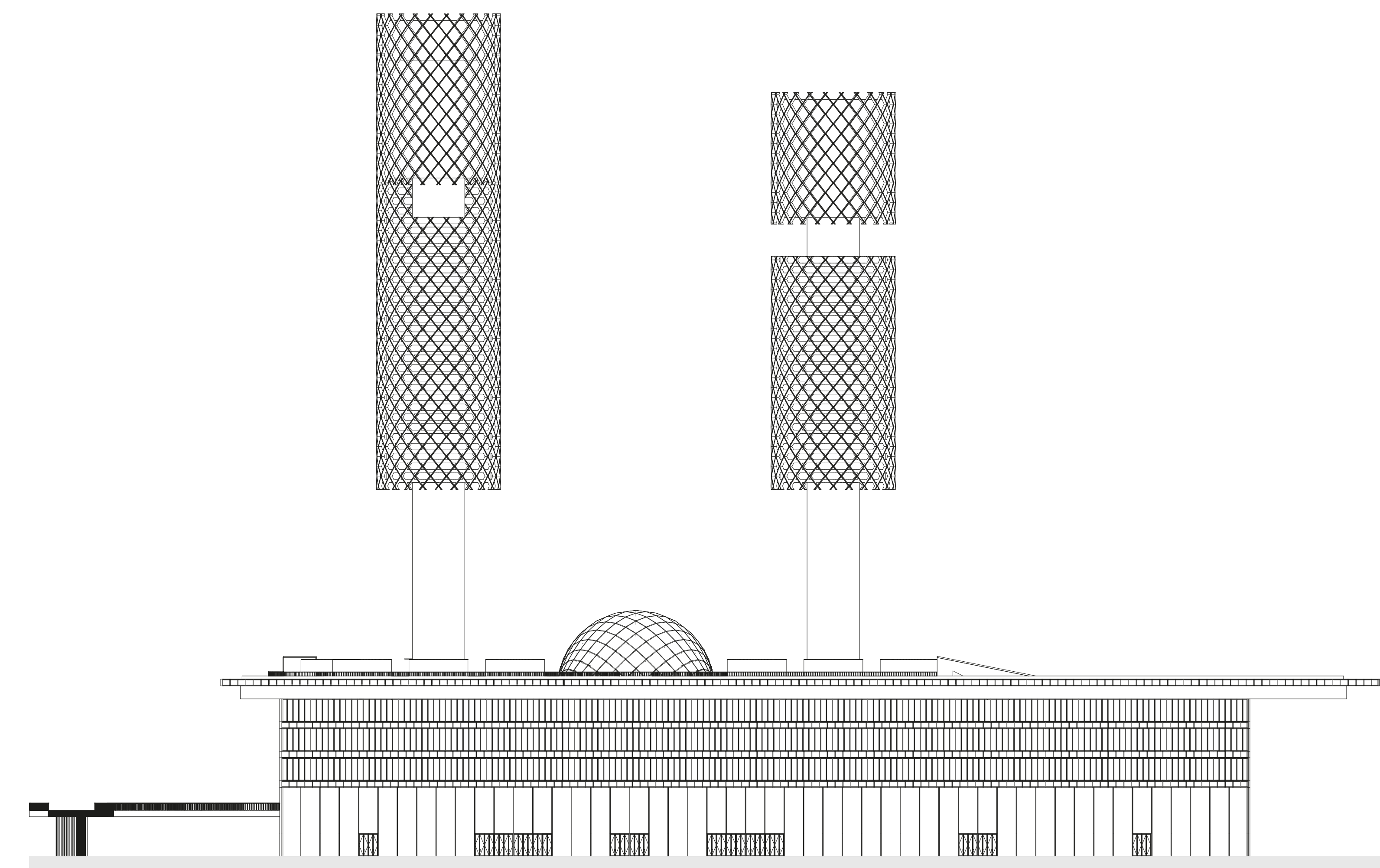
Elevation - West | 1:500
