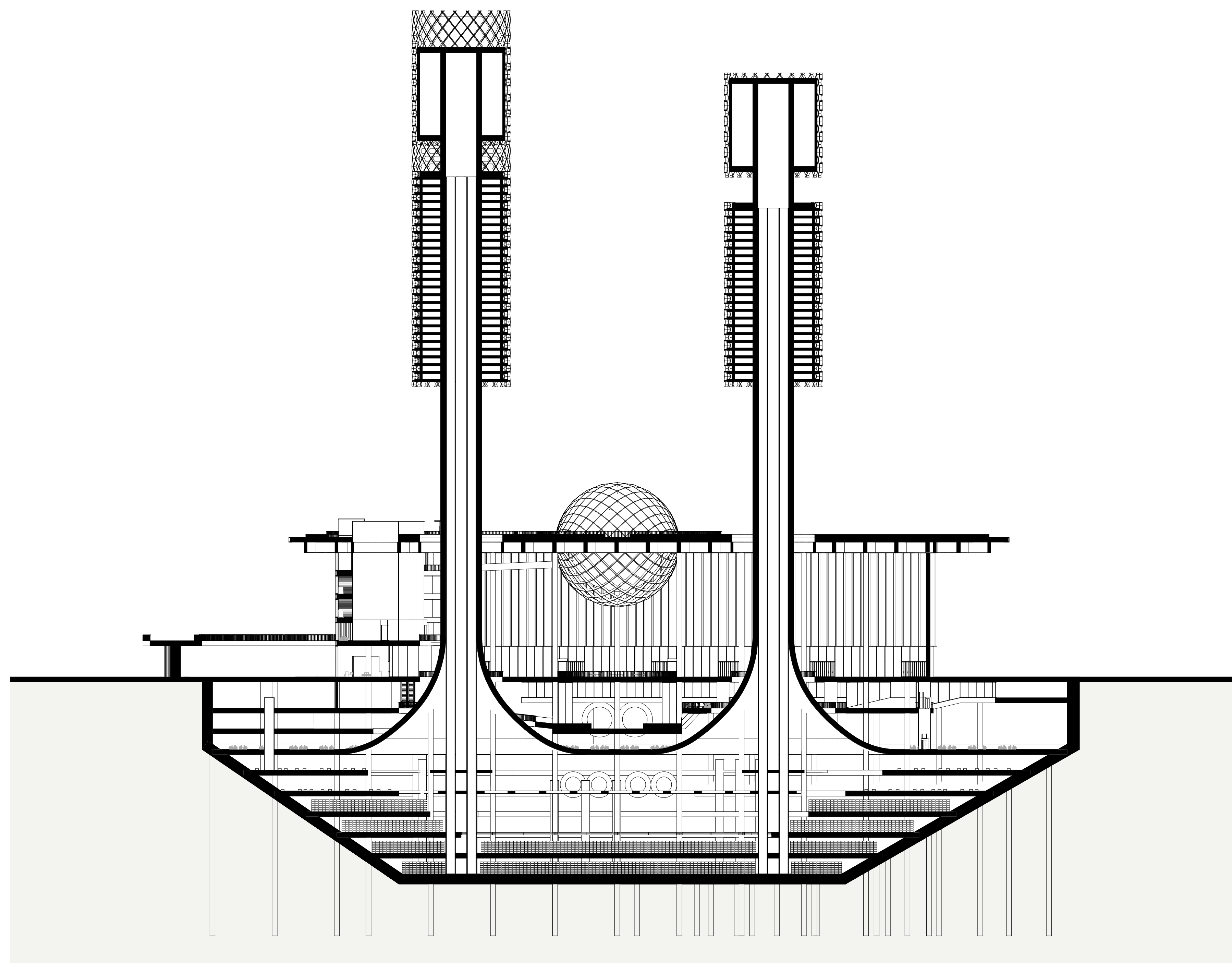
Cross section | 1:500
