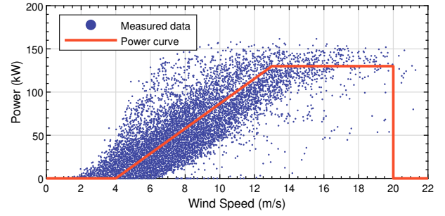
Fig. 1. Power curve for a wind turbine with: v_{\text{in}} = 4 m/s, v_{\text{rated}} = 13 m/s, v_{\text{out}} = 20 m/s and \omega_{\text{rated}} = 130 kW.
