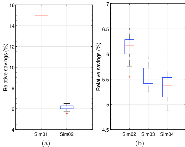
Fig. 3. Boxplot of the test user savings with respect to the expected value strategy (a) in presence of other stochastic users (b).
