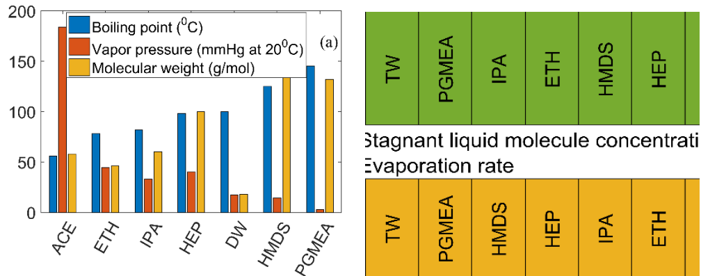
Fig. 5: (a) Physical properties related to the liquid evaporation and (b) the observed order of the increasing liquid evaporation rate and increasing liquid molecule concentration remaining on the surface, consistent with their physical properties.
