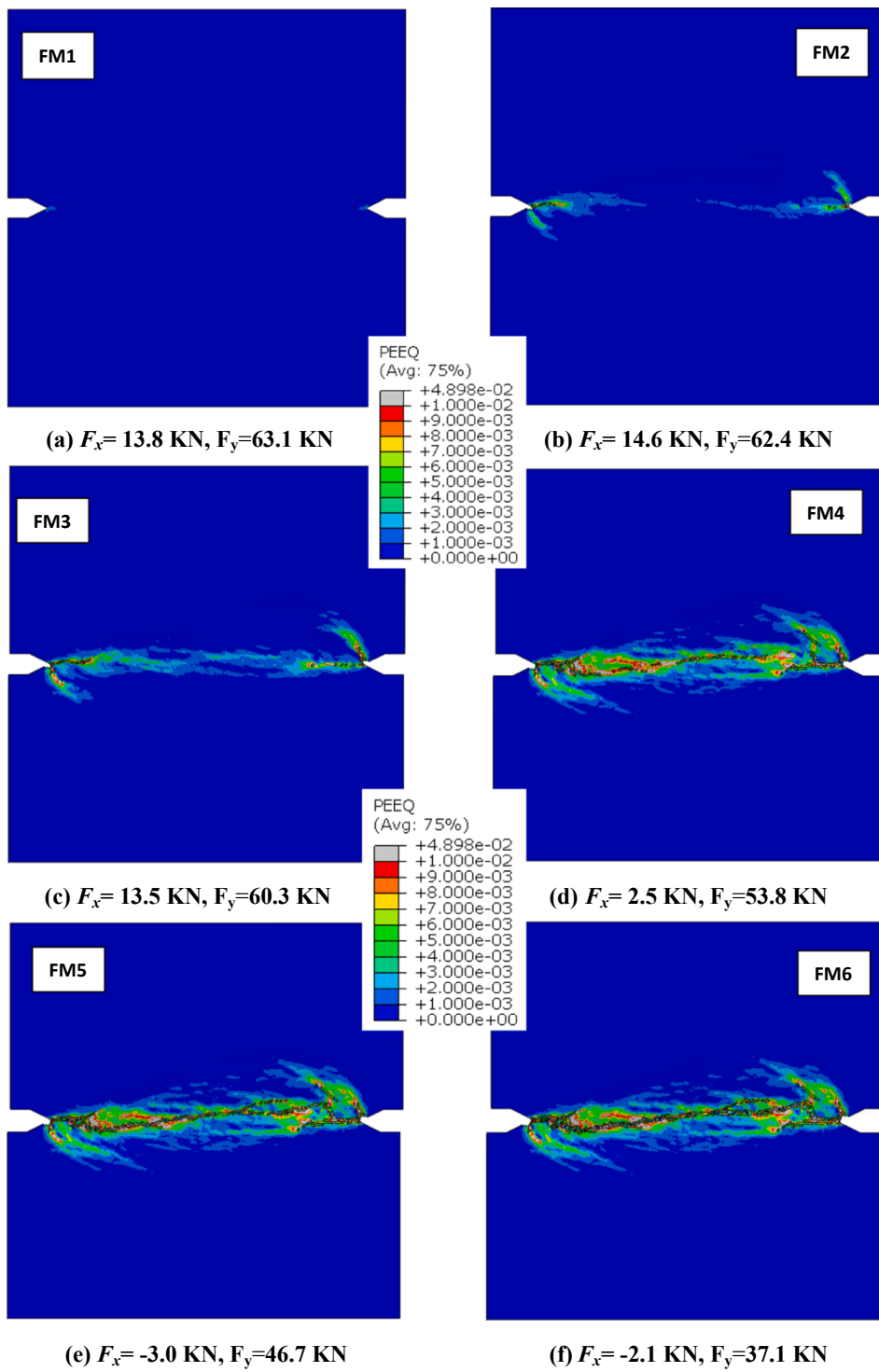
Fig. 18. Crack propagation of UHPCFRC (28 days) under tensile and shear loading.
