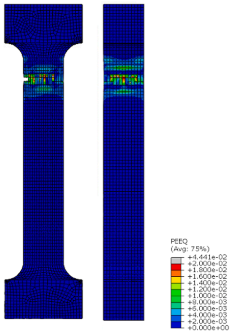
(c) UHPCFRC at 14 day (Scale=1.0)
