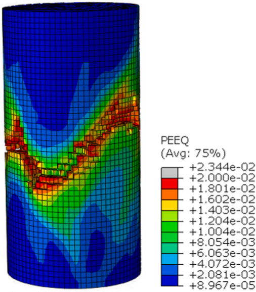
(c) UHPCFRC at 14 day (Scale=0.1)
