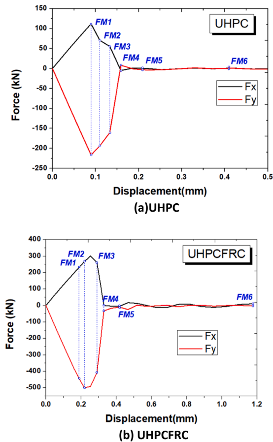
Fig. 19. Load-displacement relationship under combined compressive and shear loading.
