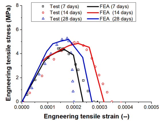
(a) UHPC
