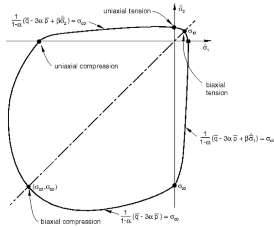
Fig. 4. Yield surface of CDP model in-plane stress [36].
