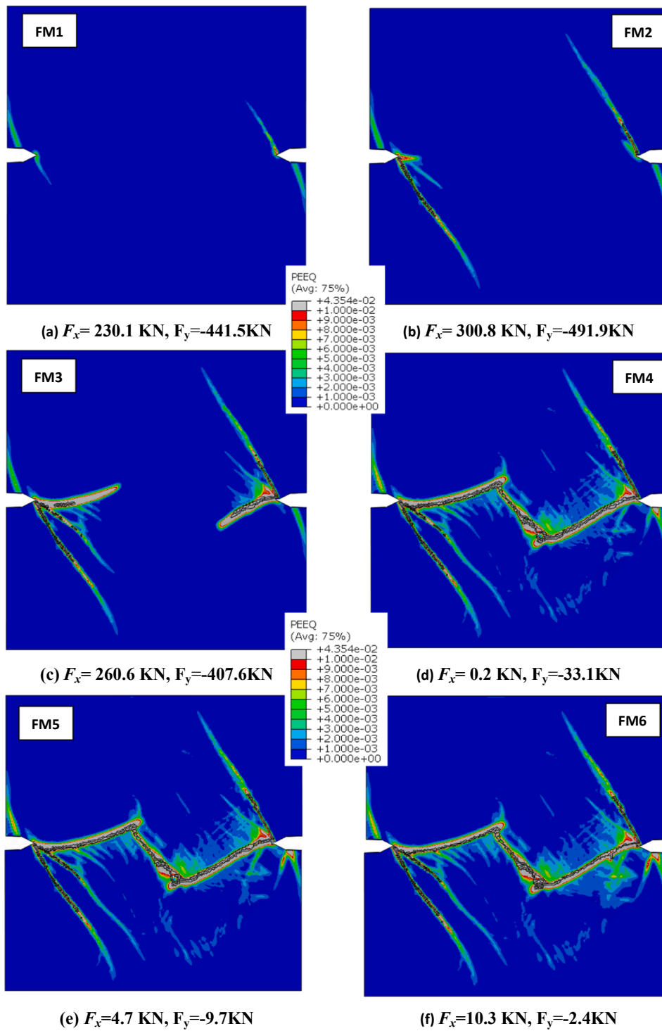
Fig. 21. Crack propagation of UHPCFRC (28 days) under compressive and shear loading.
