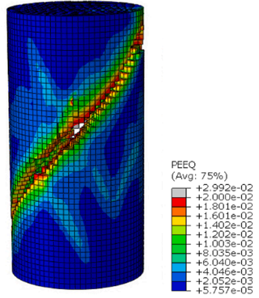
(b) UHPCFRC at 7 day (Scale=0.1)
