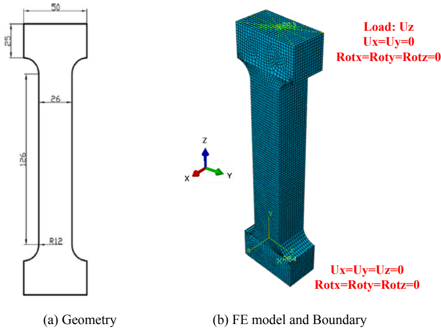
Fig. 5. Geometry and FE model of tensile specimens.
