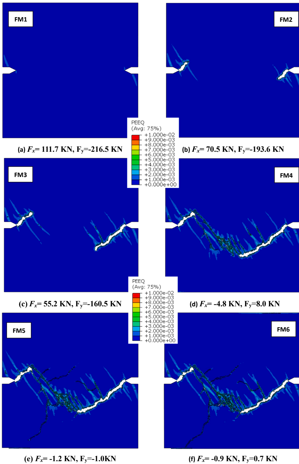
Fig. 20. Crack propagation of UHPC (28 days) under compressive and shear loading.
