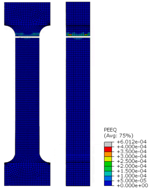
(b) UHPC (7 days) (Scale=1)
