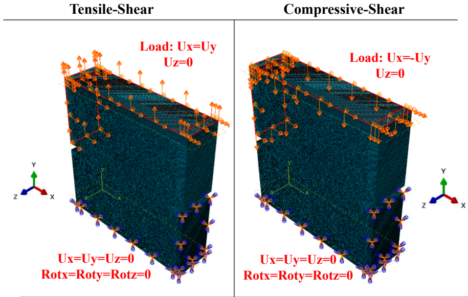
(b) Mesh and Boundary conditions
