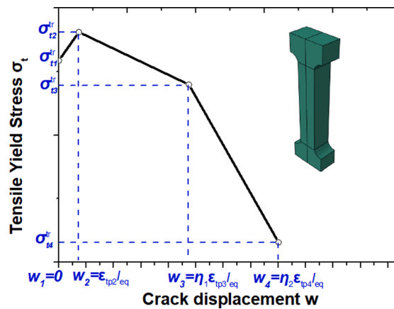
Fig. 7. Simplified tensile yield stress-crack displacement relationship.
