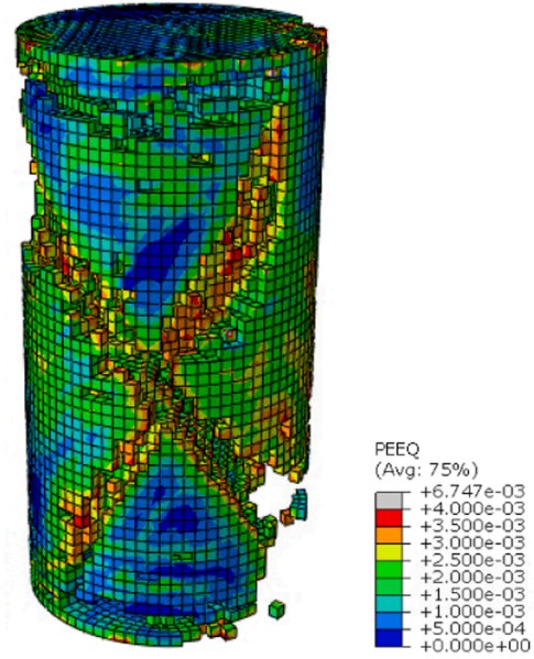
(b) UHPC (7 days) (Scale=0.1)
