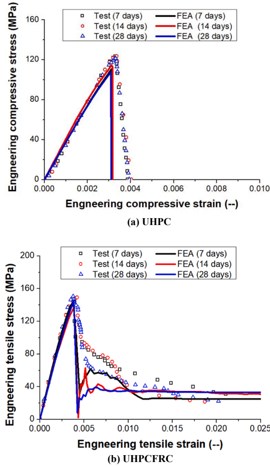
Fig. 10. Comparison between experimental and numerical results.
