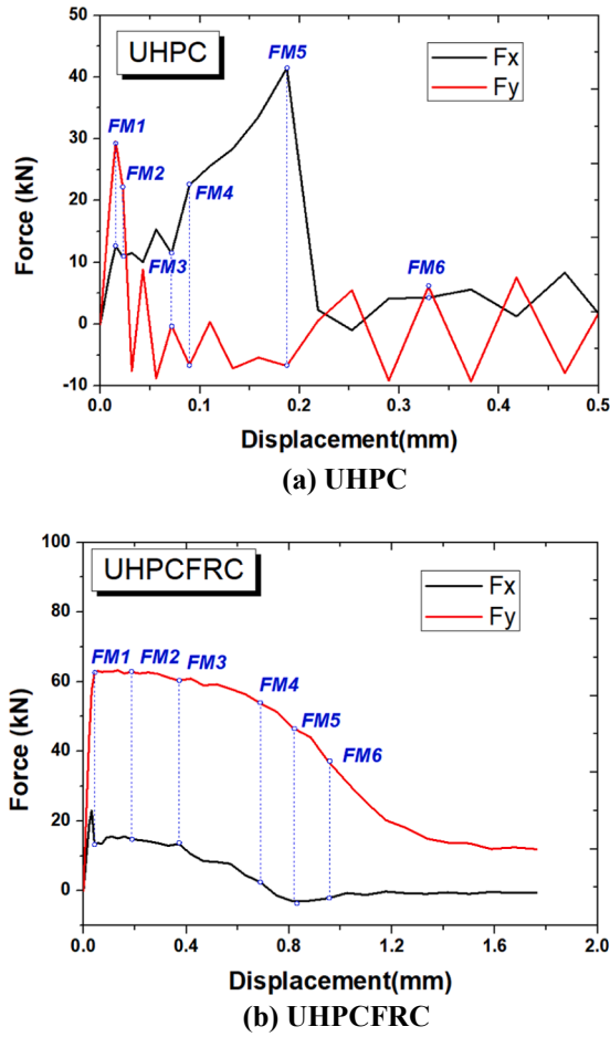
Fig. 16. Load-displacement relationship under combined tensile and shear loading.
