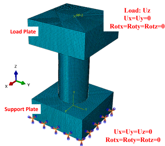
Fig. 9. FE of Compressive specimens.
