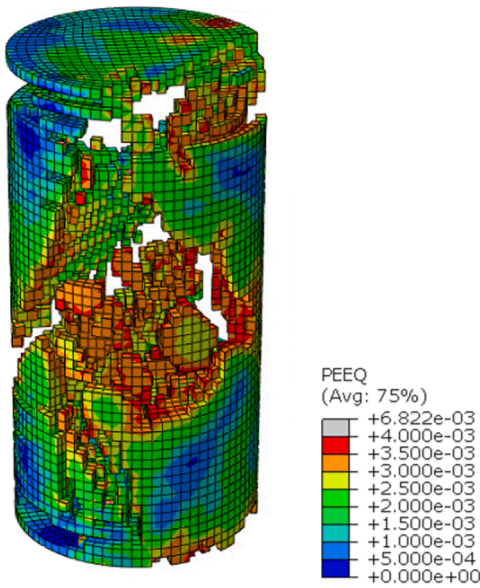
(c) UHPC (14 days) (Scale=0.1)
