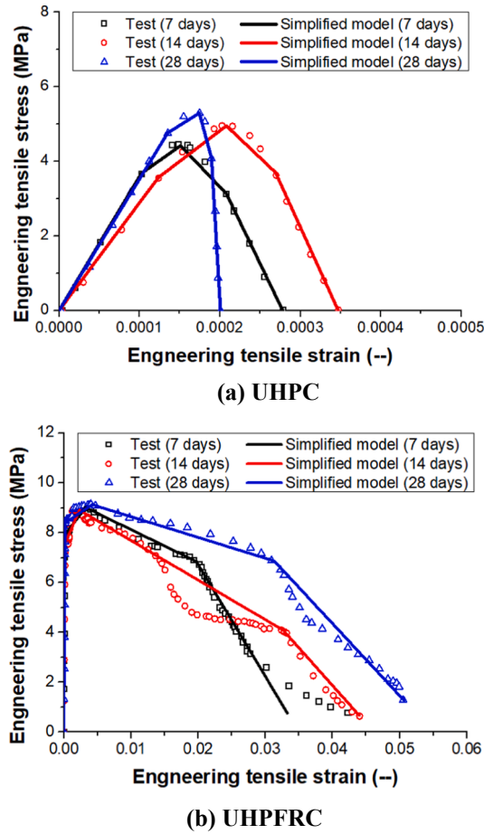
Fig. 2. Engineering tensile stress-strain comparison.
