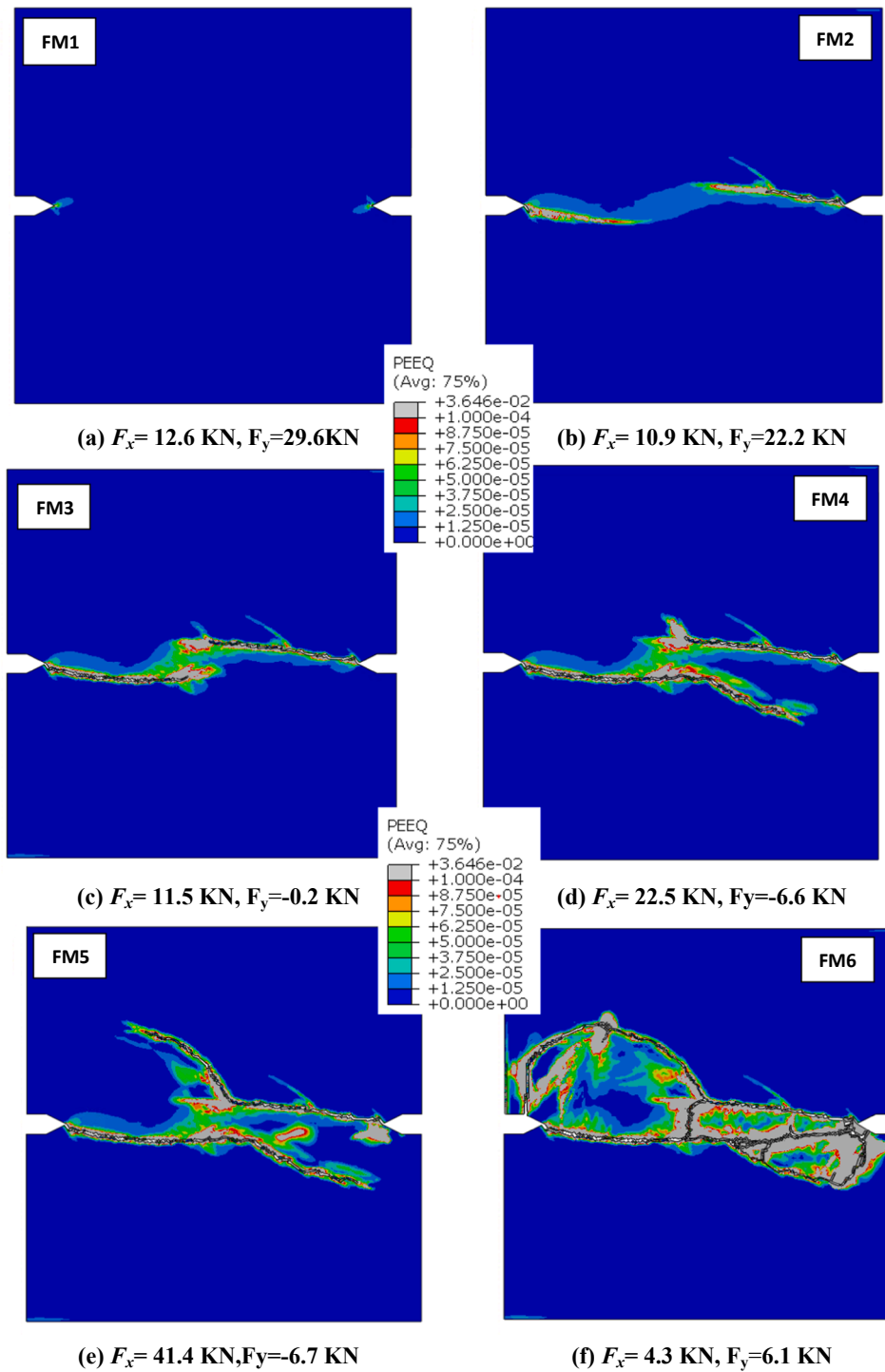
Fig. 17. Crack propagation of UHPC (28 days) under tensile and shear loading.
