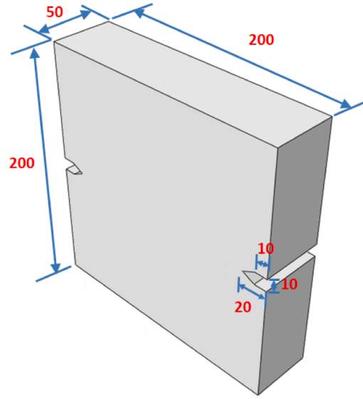
(a) Geometry of mixed mode crack propagation
