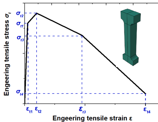
Fig. 1. Simplified engineering tensile stress-strain relationship of UHPC and UHPFRC.
