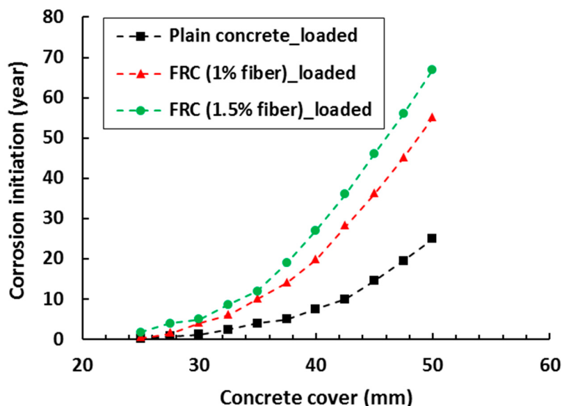
Figure 8. Predicted corrosion initiation of FRC and plain concrete at varying cover depth (adapted from [128]).
