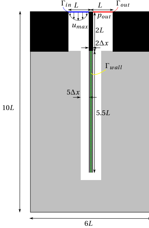
Figure 2.19: An optimization problem which minimizes pressure drop for flow around a thin wall of two elements thick. The thin wall (dark gray) is modeled using a porous formulation and its density is fixed at \underline{\alpha} , to challenge the flow model the thin wall is surrounded by a fluid non design domain (white) of five elements thick. A parabolic flow is prescribed on inlet \Gamma_{in} and a constant pressure on outlet \Gamma_{out} . The inlet/outlet are separated from the design domain by fluid pipes (white) surrounded by solid material where no flow is present (black). The optimization procedure is initialized using a completely fluid design domain (light gray).
