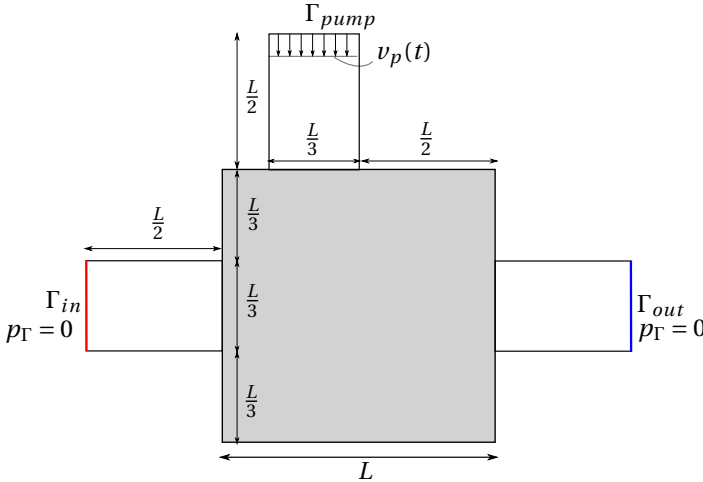
Figure 4.14: The piston pump optimization problem. At the top inlet/outlet, a fluctuating velocity is prescribed and at the red inlet and blue outlet only reference pressures are prescribed. The white domains are non-design areas, and in the gray domain, the material layout is optimized.
