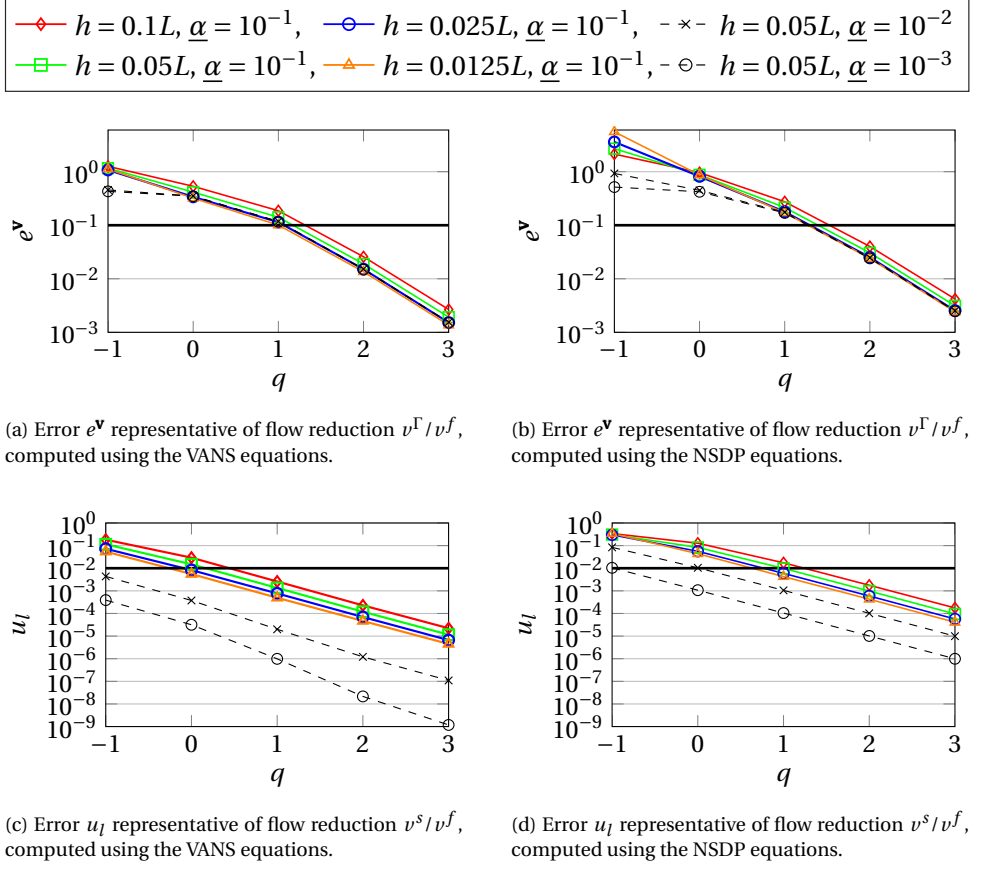
Figure 2.14: The errors e^v and u_l for low Re^e in the problem as illustrated in Figure 2.12 using the parameters from Table 2.3 computed using varying h and \alpha . The horizontal solid black lines indicate the maximum allowable errors e^v \approx 10^{-1} and u_l < 10^{-2} for optimization, and are used to select appropriate optimization parameters q and \alpha .
