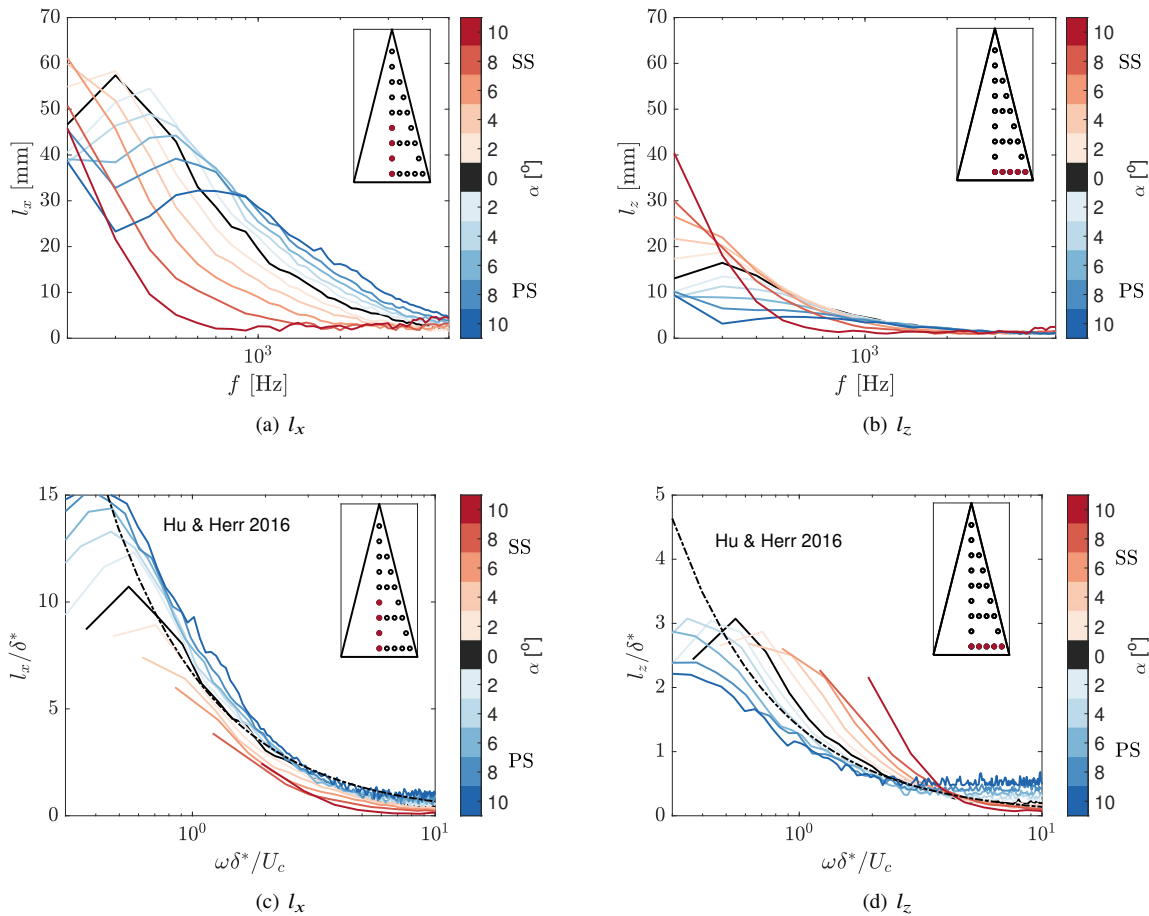
Fig. 8 Variation of the stream (a and c) and spanwise (b and d) correlation length at the root of the serration with frequency and Strouhal number for different angles of attack ( Re = 2,000,000 ).
