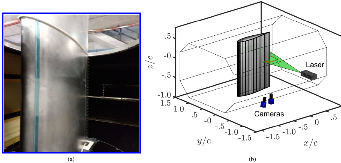
Fig. 1 BANC NACA 63-018 2D wing model mounted inside the LTT wind tunnel with Kevlar test section (a) and illustration of the model, test section and PIV setup (b).
