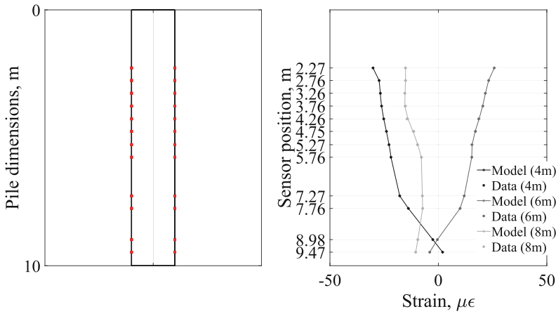
Fig. 4. Mode-matching based fit of the axial strain data of the VH pile at three different penetration depths (4 m, 6 m and 8 m).
