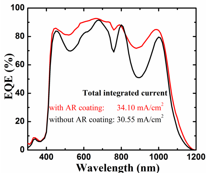
Fig. S4 The sum of the EQEs from the top perovskite and bottom silicon sub-cells.
