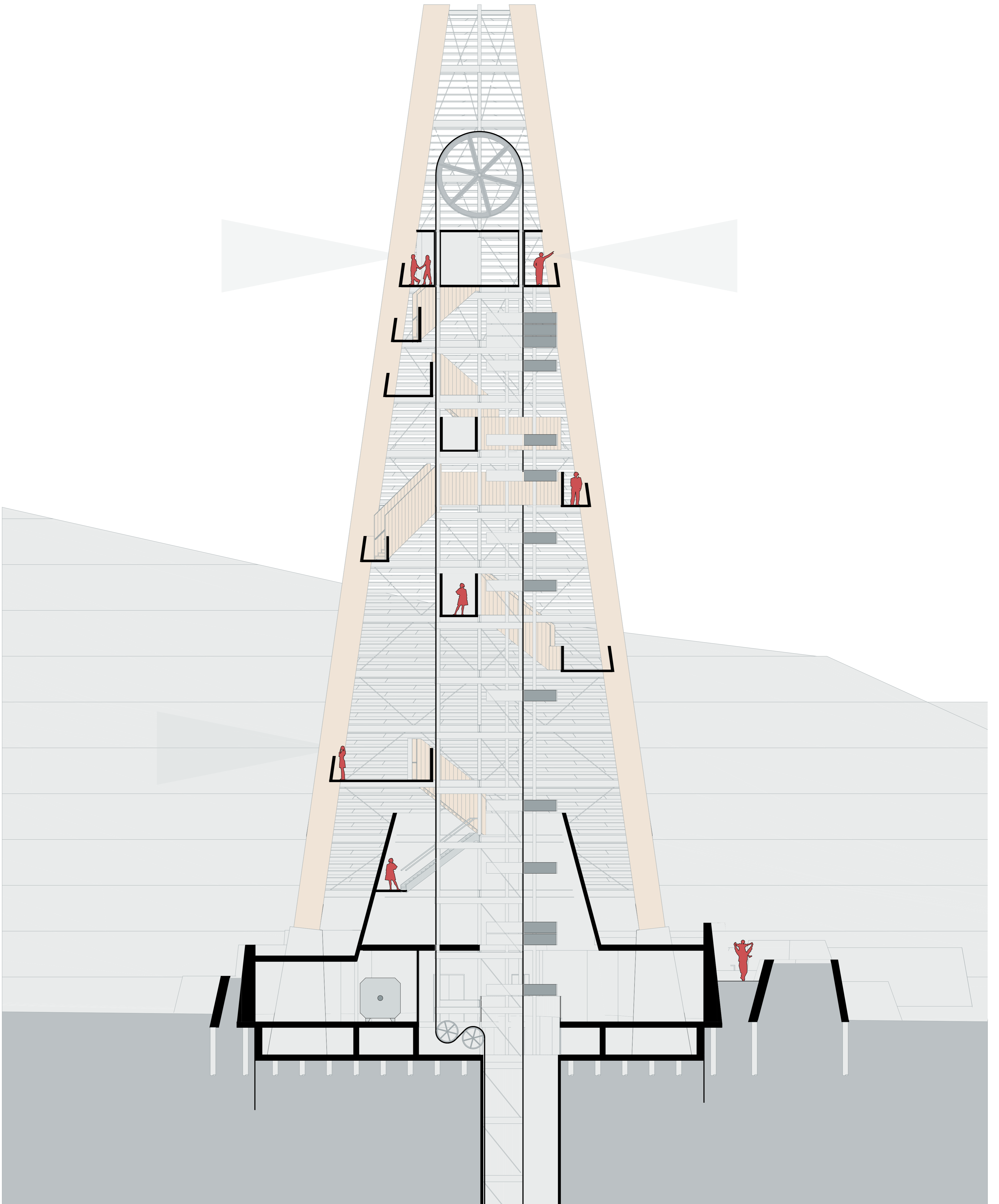
longitudinal section - storage tower 1
