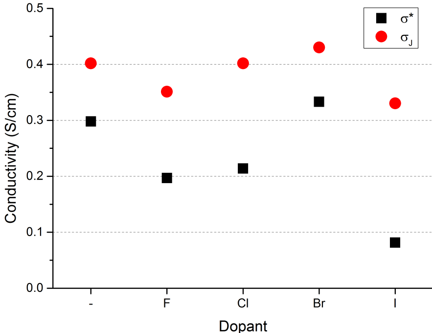
Figure 7: The conductivities for 4% Na-vacancy concentration without (-) and with halogen doping from MD-simulations of the cubic phase at 525 K based on the MSD ( \sigma^* ) and mean Na1→Na1 jump rates ( \sigma_J ).
