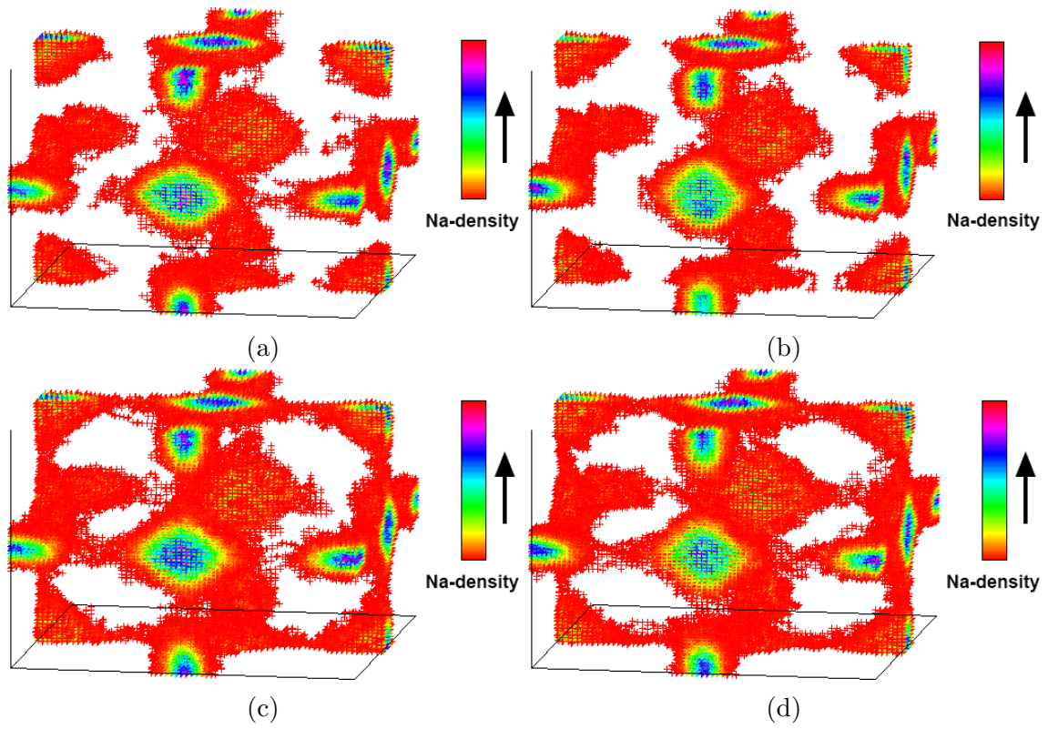
Figure 2: The Na-distribution during a 100 ps. MD-simulation at 525 K for (a) cubic \text{Na}_3\text{PS}_4 , (b) tetragonal \text{Na}_3\text{PS}_4 , (c) cubic \text{Na}_{2.94}\text{PS}_4 , and (d) tetragonal \text{Na}_{2.94}\text{PS}_4 .
