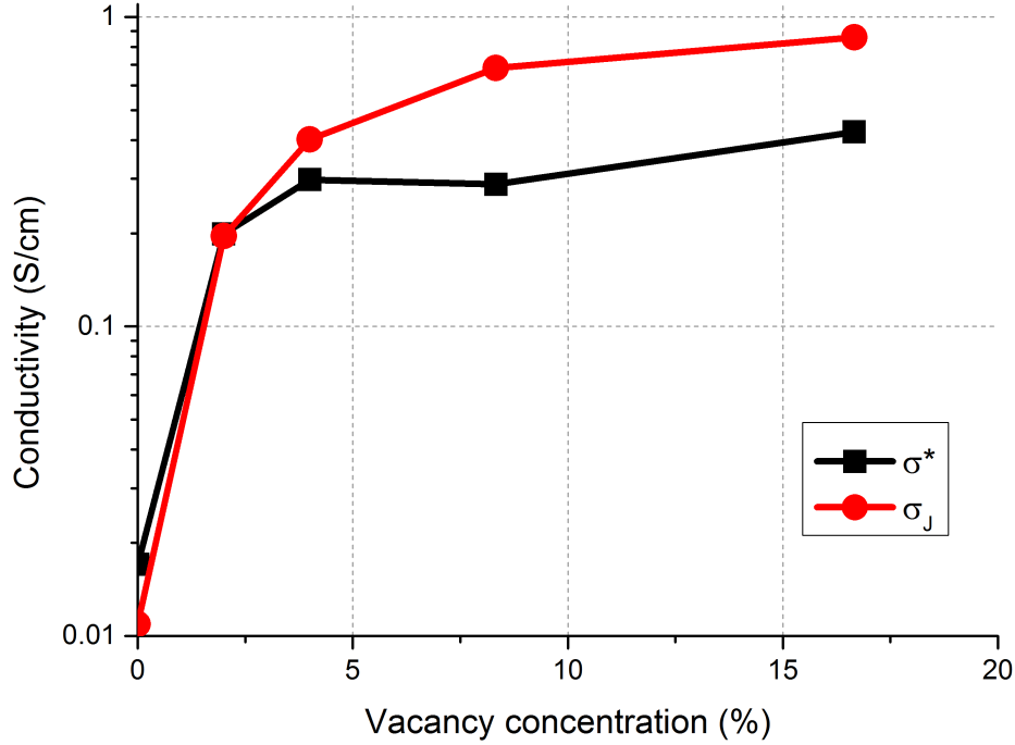
Figure 4: The conductivity, based on the tracer conductivity ( \sigma^* ) and on the mean Na1→Na1 jump rate ( \sigma_J ), versus vacancy concentration for the cubic phase at 525 K.
