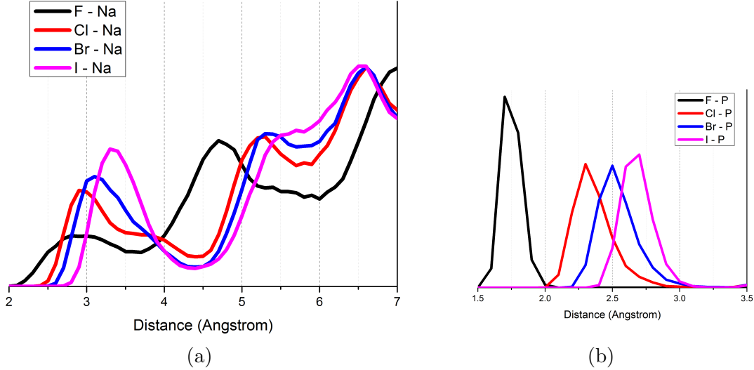
Figure 8: The (a) X-Na distribution between 2 and 7 Å, and (b) the X-P distribution between 1.5 and 3.5 Å from the MD-simulation of cubic \text{Na}_{2.88}\text{PS}_{3.88}\text{X}_{0.12} (X = F, Cl, Br, I) at 525 K.
