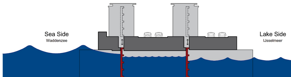
Fig. 2. Impression of an existing flood gate complex in the Afsluitdijk, closed during high water level at the sea side. Standing wave impacts can occur in this flood gate complex at the sea side due to extreme incident waves (global impact on the overhang), and/or at the lake side due to moderate incident waves (global impact on the overhang or local impact on gate reinforcements).
