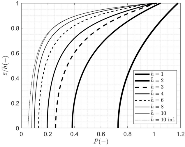
(a) Pressure-impulse profile at wall for \beta = 1 .
