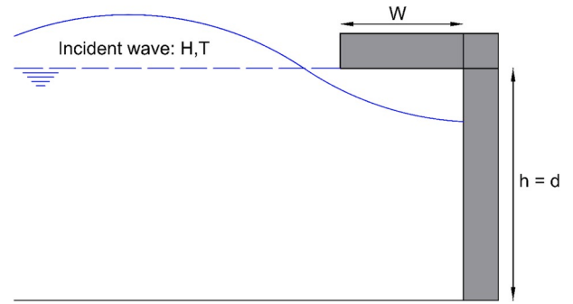
Fig. 3. H : incident wave height; T : incident wave period; d : still water depth; h : overhang height; W : overhang width.
