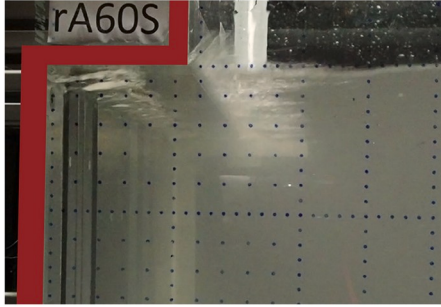
(a) Impact Type I: for AS and CS. Intermediate entrapped air, near the wall
