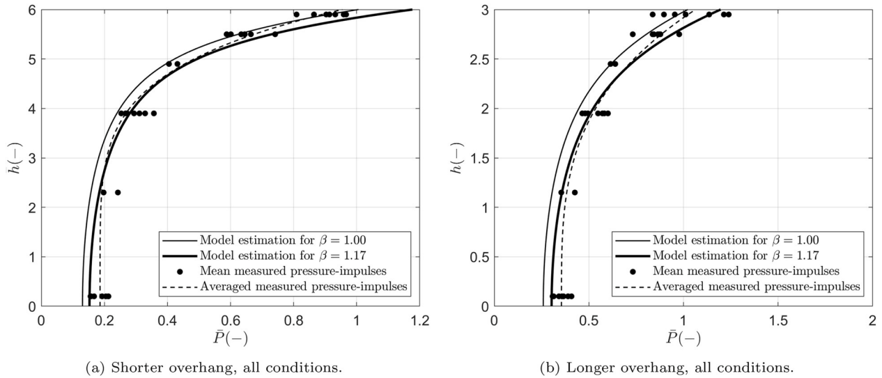
Fig. 15. Summary dimensionless pressure-impulse profile \bar{P} .
