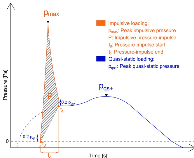
Fig. 9. Pressure-impulse calculation method.
