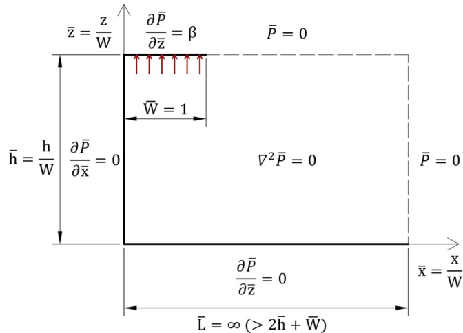
Fig. 4. Dimensionless pressure-impulse model for a vertical impact on a horizontal overhang (based on (Wood and Peregrine, 1996)).
