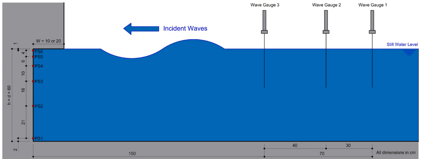
Fig. 8. Illustration of test setup and instrumentation. Note that all dimensions are in centimetres (cm).
