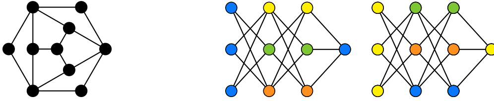
Figure 3: Left: A graph G for which \text{diam } \mathcal{C}_3(G) < \text{diam } \mathcal{C}_4(G) . Right: Two [4]-colourings of G (drawn differently from the figure on the left) that in \mathcal{C}_4(G) lie at distance 17.
