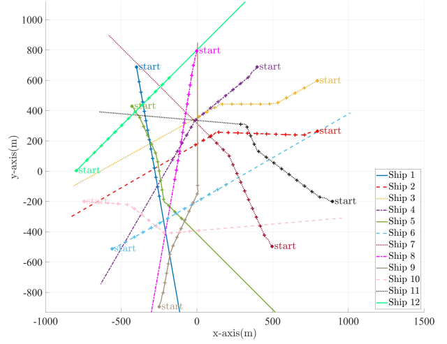
(b) Simulated ship trajectories with Obj_1 .
