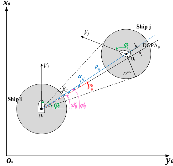
Figure 5: A two ships encounter case as an illustrative example of collision risk parameters.
