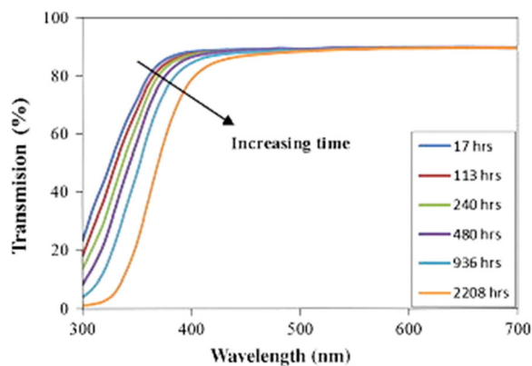
Figure 15. Transmission of light in photo thermally aged BPA-PC [54], reproduced with permission from Elsevier.
