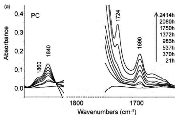
Figure 25. Changes in the carbonyl region of IR spectra of thermo-oxidised PC film at 170°C [49].
