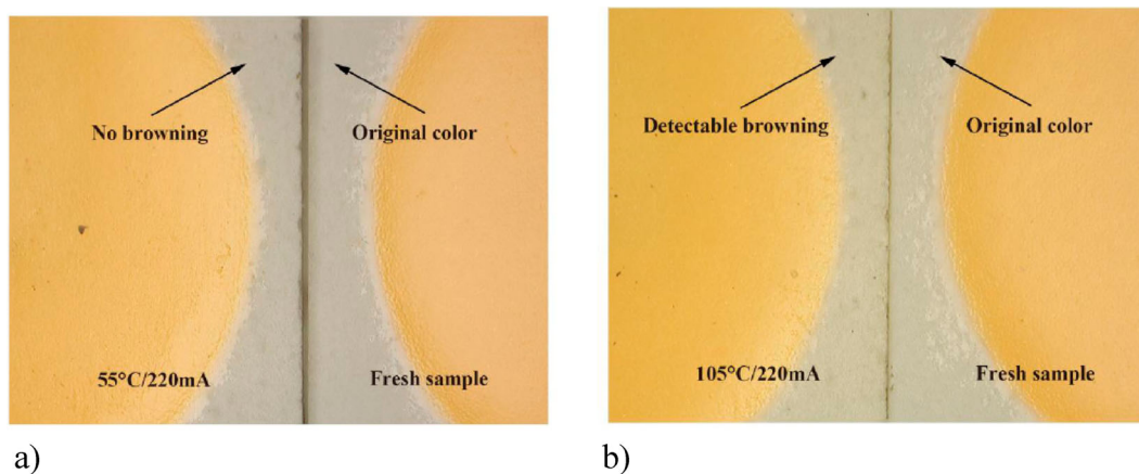
Figure 34. Influence of ageing at (a) 55°C and (b) 105°C for 6000 h on the discolouration of epoxy in LED [29], reproduced with permission from authors.
