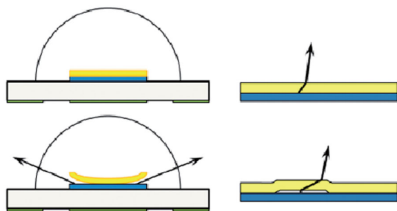
Figure 17. Edge and centre phosphor delamination in LED package [164].
