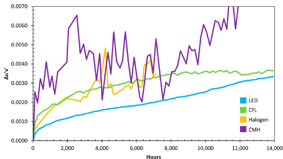
Figure 14. Average change in the chromaticity of different light sources with time [205].
