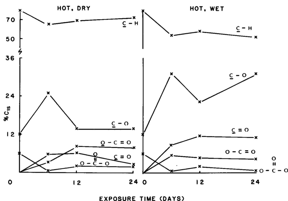
Figure 29. C1s X-ray photoelectron spectra components assigned from curve fits for photo-aged PC sample in wet/dry condition.
