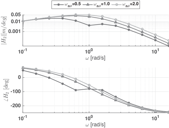
Fig. 6: Surge frequency response function due to pitch input, test 2 of the OMCT.
