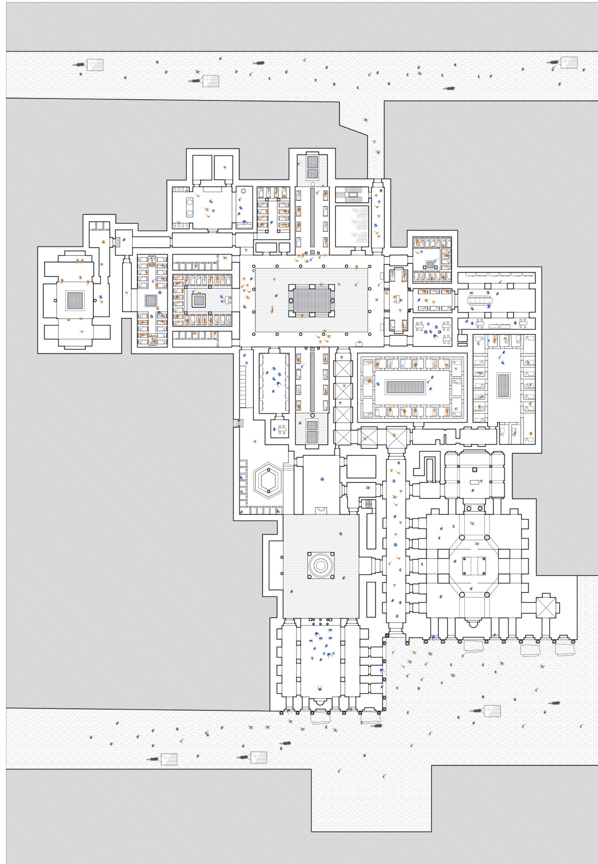
BIMARISTAN AL QALWUN IN CAIRO
