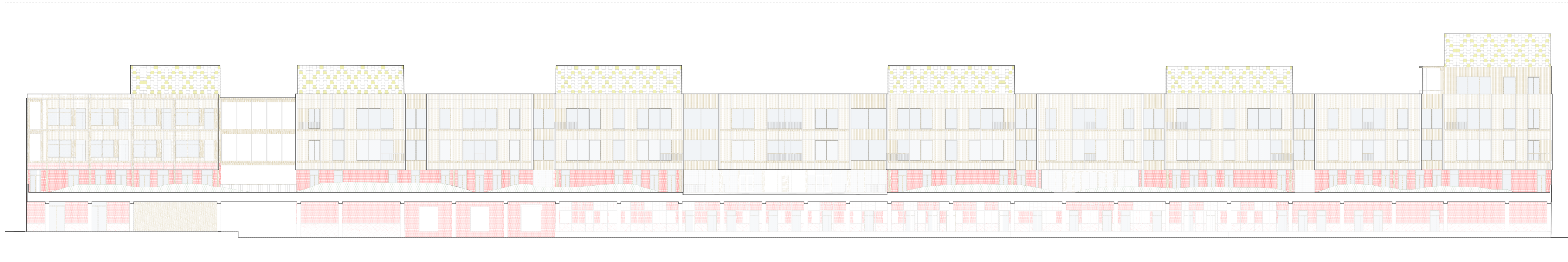
ELEVATION - SOUTH - MAASBOULEVARD
