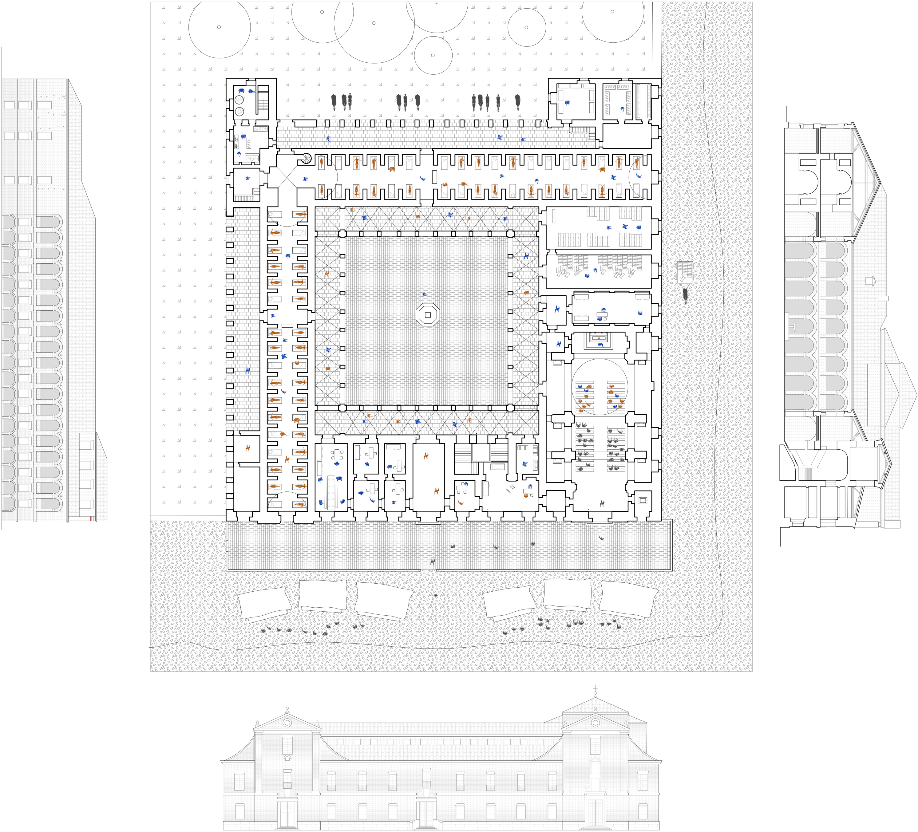
HOSPITAL SIMON RUIZ IN MEDINA DEL CAMPO
