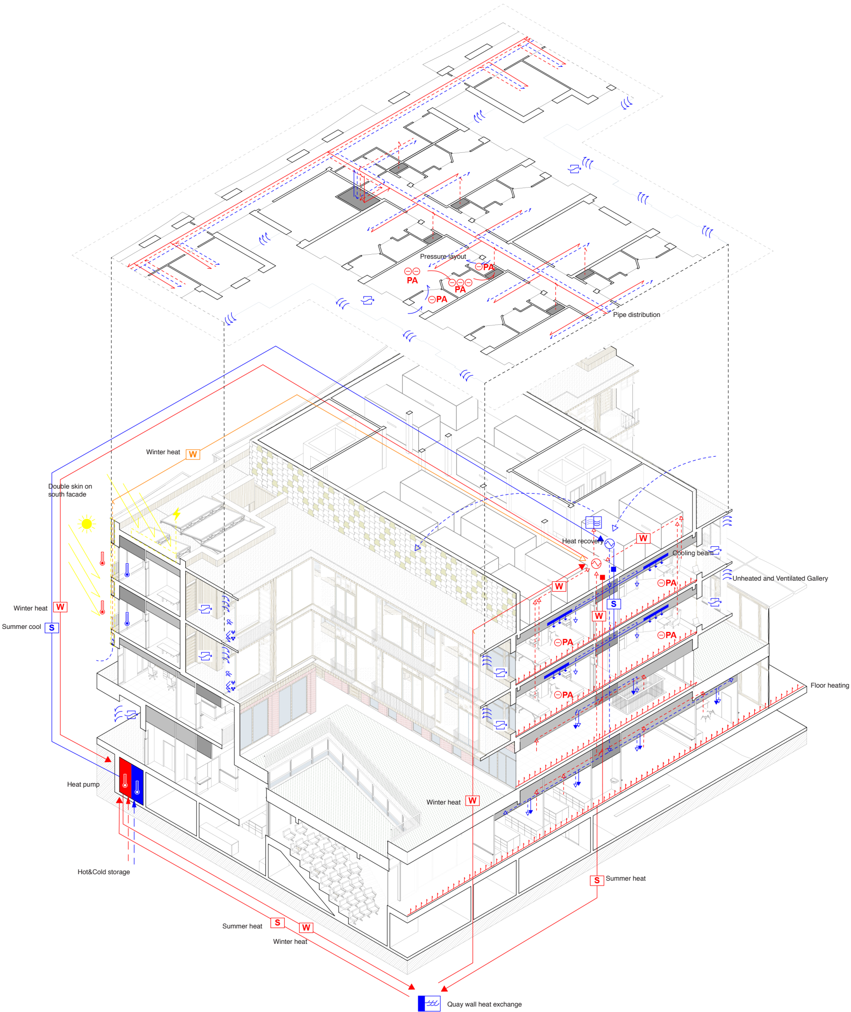
AXONOMETRY - CLIMATE
