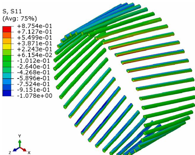
Fig. 29. Contour plot of stress of wires in X1-direction for \kappa_G = 0.2e - 3 \text{ mm}^{-1} from the full-scale model.
