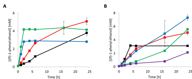
Figure 2. Influence of the reaction pH (A) and sulfite concentration (B) on the plant-SO – rAaeUPO cascade performance. General conditions: [PSO] = 100 nM, [ rAaeUPO ] = 500 nM, [Na 2 SO 3 ] 0 = 10 mM, [ethylbenzene] 0 = 100 mM in a 50 mM Bis-Tris buffer at pH 7.0. Reactions were performed in duplicates, with reaction volumes of 250 μl, in a thermos shaker at 30 °C and 500 rpm. A: performance at pH 6.5 (black), pH 7.0 (red), pH 7.5 (blue) or pH 8.0 (green). B: Sodium sulfite concentration of 5 mM (black), 10 mM (red), 20 mM (blue), 50 mM (green) or 100 mM (purple).
