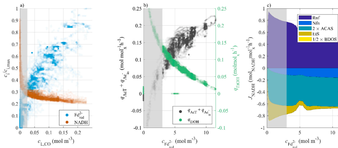
Fig. 7. Mechanism towards ethanol production in a lifeline. a) The relationship between the concentration of electron carriers \text{Fd}_{\text{red}}^{2-} (blue) and NADH (orange) is shown and their corresponding c_{\text{L,CO}} ( c_{\text{Fd}_{\text{red}}^{2-},\text{max}} = 11.5 \text{ mol m}^{-3} , c_{\text{NADH},\text{max}} = 0.04 \text{ mol m}^{-3} ). b) the relationships between acetate production (extracellular + intracellular) (black) and ethanol production (green) with c_{\text{Fd}_{\text{red}}^{2-}} . c) the rates of NADH production (Rnf, darkblue) and consumption (Nfn, light blue; ACAS, green; Ethanol Synthesis, gold; BDO Synthesis, yellow) as function of c_{\text{Fd}_{\text{red}}^{2-}} . The scatters mark temporal observations during a lifeline (between 100 and 1000 s), and their density denotes the probability of occurrence. Figure c) is an energy balance that can be made since \tau_{\text{NADH}} \ll \tau_{\text{Fd}_{\text{red}}^{2-}} . Shaded areas mark zones with c_{\text{L,CO}} < 0.025 \text{ mol m}^{-3} .
