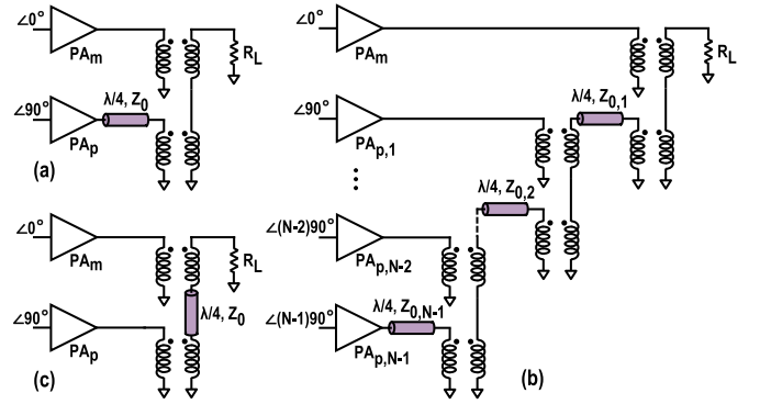
Fig. 2. Schematic of (a) conventional two-way SDC, (b) N -way SDC proposed by [21], and (c) modified schematic of the conventional two-way SDC.
