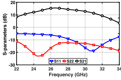
Fig. 14. Measured small-signal S-parameter.
