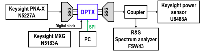
Fig. 13. Simplified block diagram of the measurement setup.
