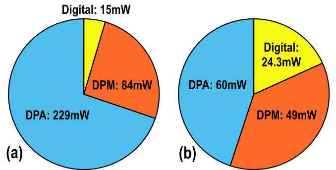
Fig. 19. Measured power breakdown when the TX generates (a) CW signal at its peak power and (b) 64-QAM 300MHz modulated signal with \sim 6.7 dB PAPR.
