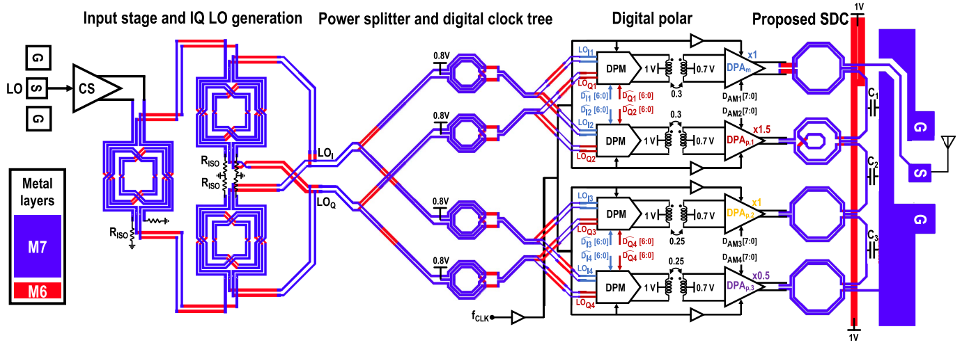
Fig. 7. Block diagram of the proposed DPTX.
