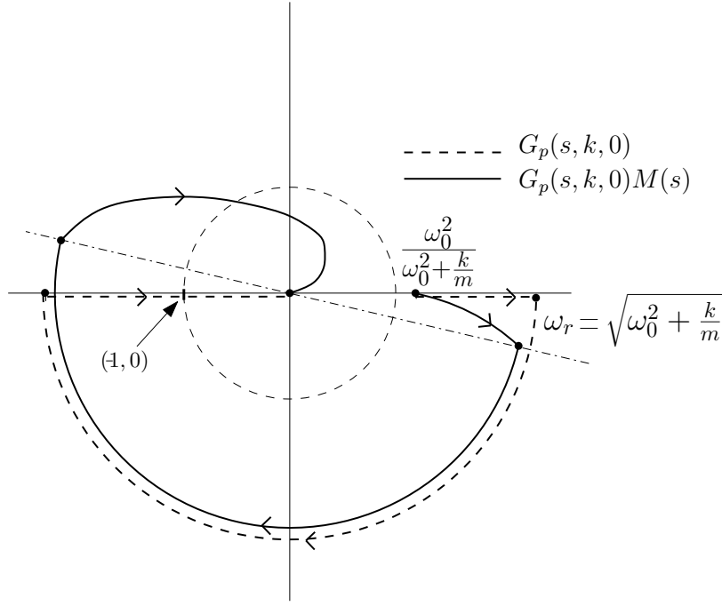
Figure 5: First path of the Nyquist diagram of the robot (with and without including the inner-loop dynamics).
