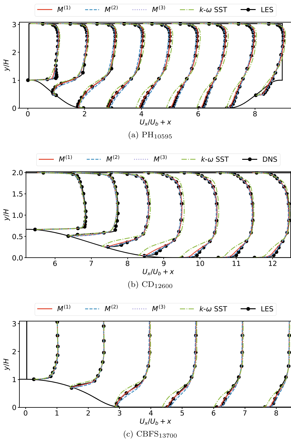
Fig. 7 Predicted stream-wise velocity
