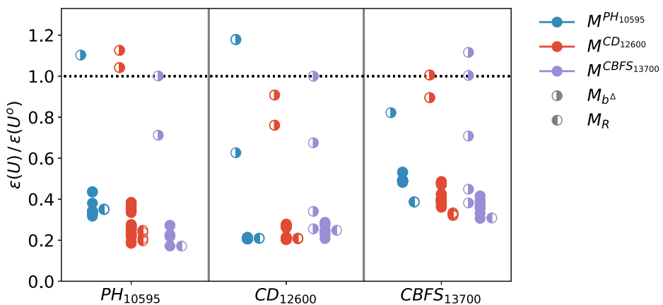
Fig. 5 Mean-squared error of velocity vector of each correction model normalised by the mean-squared error of the baseline k\text{-}\omega SST. The colour indicates on which high-fidelity data the models have been identified. Full circles represent simulations using both corrections, while left-/right-filled circles represent simulations using only correction for R or b_{ij}^\Delta respectively
