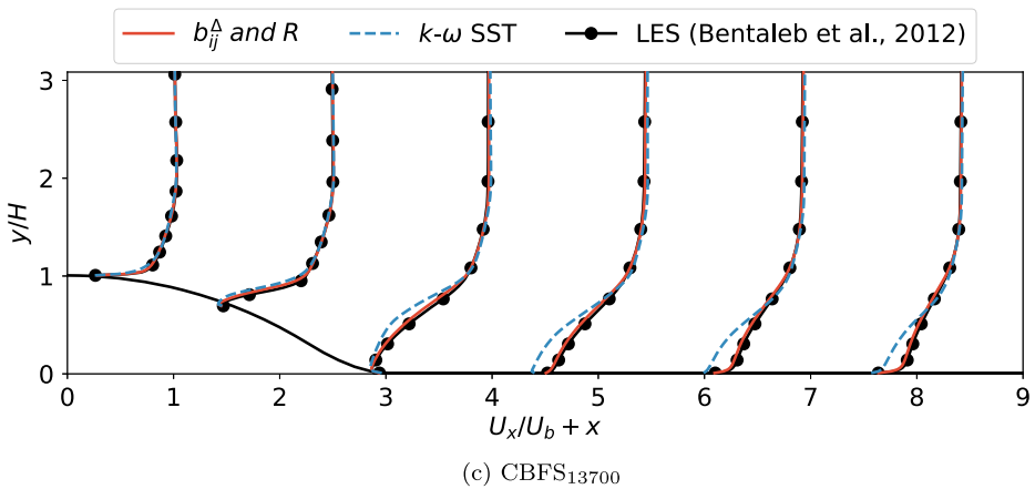
Fig. 2 Stream-wise velocity component for propagated model-form error acquired using k -corrective-frozen-RANS
