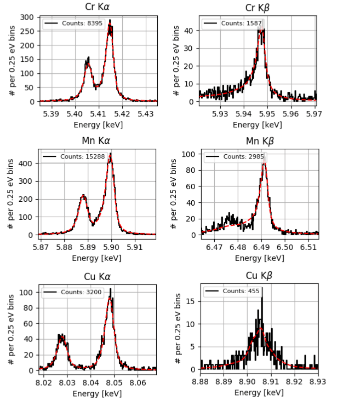
Fig. 3. Preliminary fit of the main K \alpha and K \beta lines (generated by MXS and internal ^{55}\text{Fe} X-ray source) acquired by Px1 biased at 1.1 MHz.
