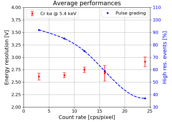
Fig. 9. Energy resolution of the Cr-K \alpha line (5.4 keV) as a function of the count rate. Red points are average values over the three pixels biased at 1.1, 2.7 and 4.6 MHz. The blue points indicate the fraction of good events used to fit the spectra. Consider that on the X-IFU 30 cps/pixel roughly correspond to 1 Crab flux.
