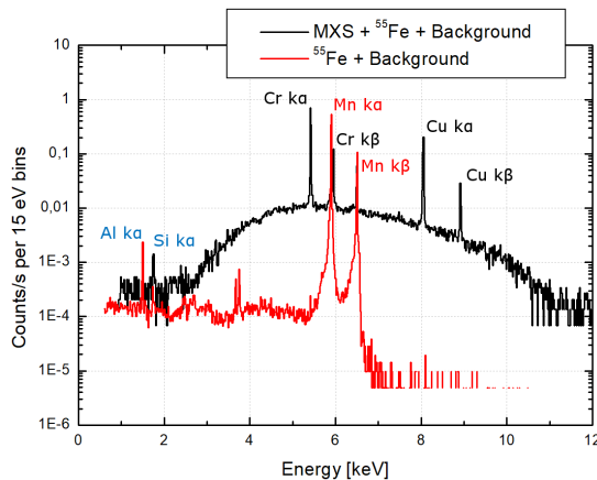
Fig. 2. Energy spectrum measured by Px8 (2.7 MHz bias frequency) with the MXS turned ON (black curve) and OFF (red curve).
