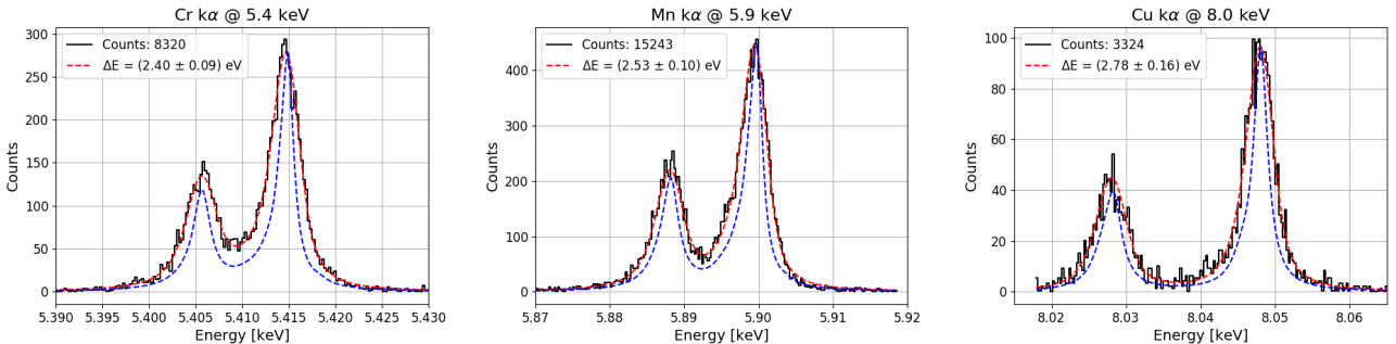
Fig. 5. Best fit to data (red lines) for each detected K \alpha line (MXS and internal 55Fe X-ray source) for Px1 biased at @ 1.1 MHz. The lines intrinsic shape (blue lines) has been described according to [16].
