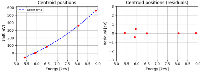
Fig. 4. (Left) Measured energy shift of the detected lines as a function of the energy, as obtained by the preliminary fit (data from Px1 biased at 1.1 MHz). The blue dashed lines is a 3th order polynomial fit of the data. (Right) Residuals of the 3th order polynomial fit. The fit accuracy is better than 0.5 eV.
