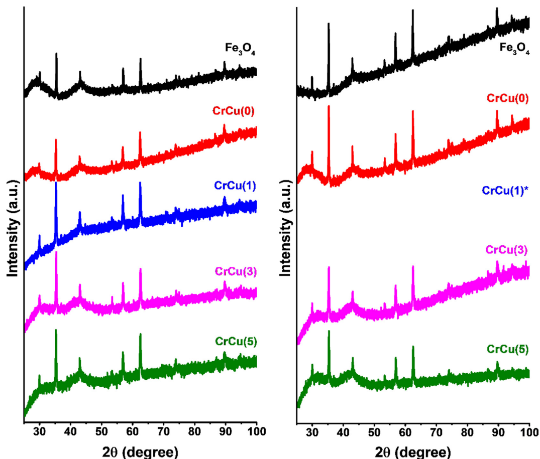
Fig. 4. XRD patterns after treatment under HTS conditions for 96 h at 2 bar (left) and 25 bar (right). *no XRD pattern for \text{CrCu}(1) after 25 bar was recorded.
