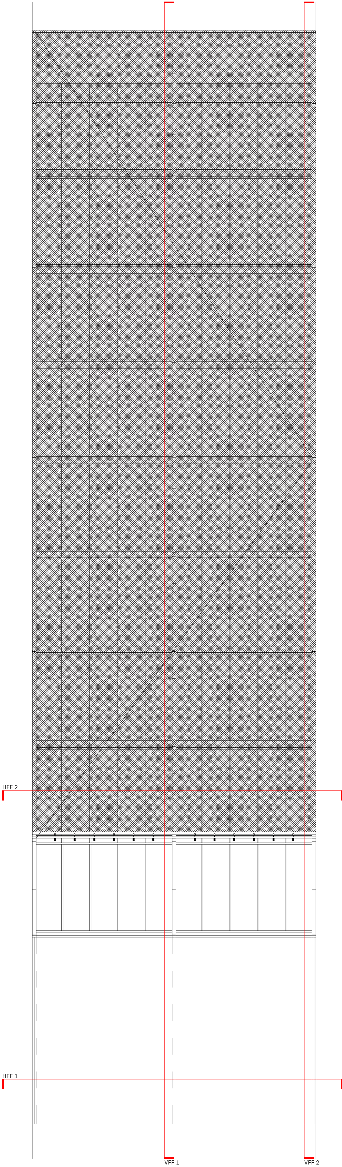
outer facade fragment elevation
