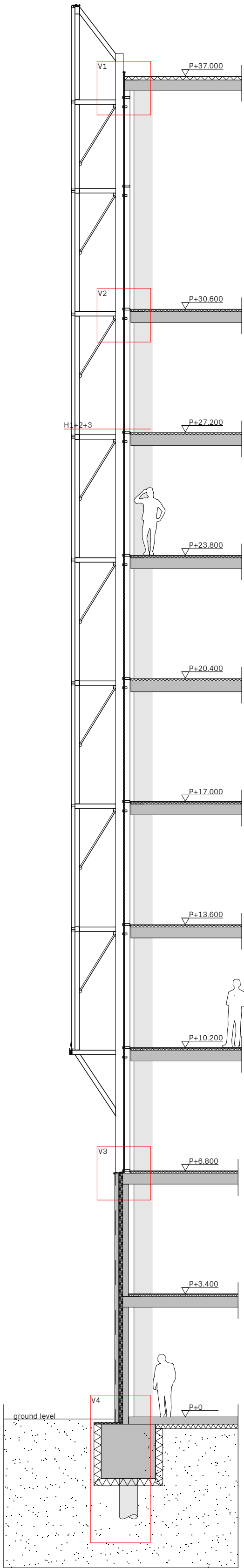
vertical facade fragment section [VFF] 2
