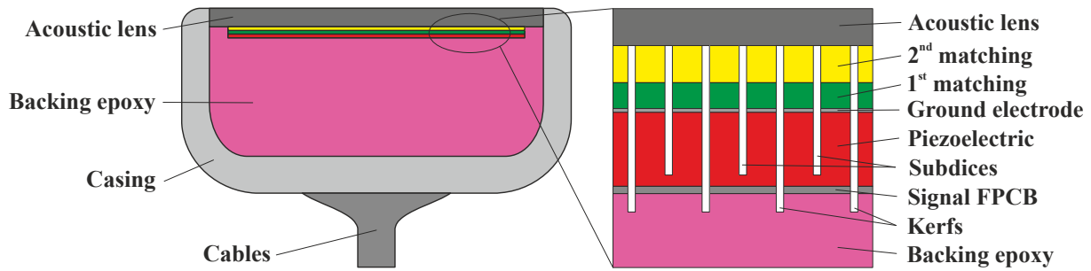
Figure 1.3. Schematic structure of a 1D array
