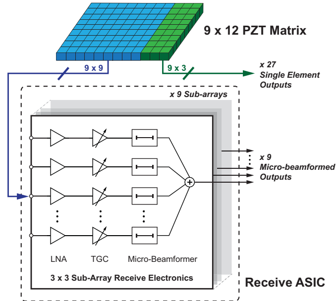
Figure 7.2. The architecture of the prototype matrix transducer.
