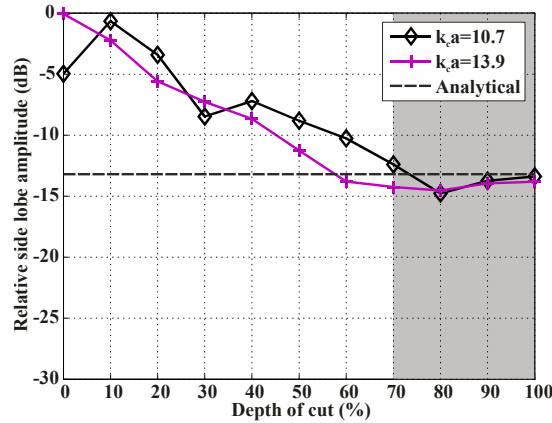
Figure 2.9. Relative sidelobe level versus the relative depth of the Subdicing cut. Data are shown for elements of size a = 180 \mu\text{m} ( k_c a \approx 10.7 ), and a = 240 \mu\text{m} ( k_c a \approx 13.9 ). In the shaded area, almost no further improvements are obtained. The dashed line is the analytical sidelobe level.
