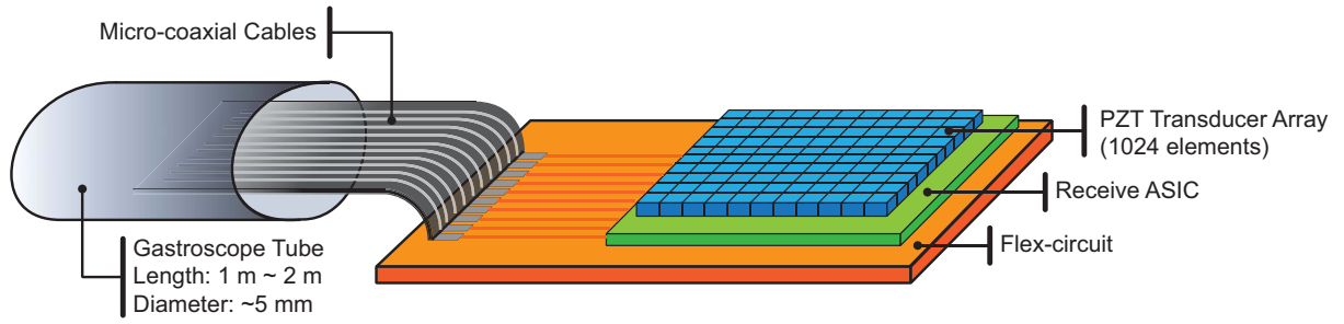
Figure 7.1. Schematic diagram of the envisioned full TEE probe.
