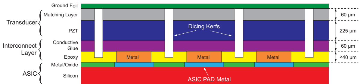
Figure 7.3. PZT-on-CMOS integration scheme with labeled layer thicknesses.
