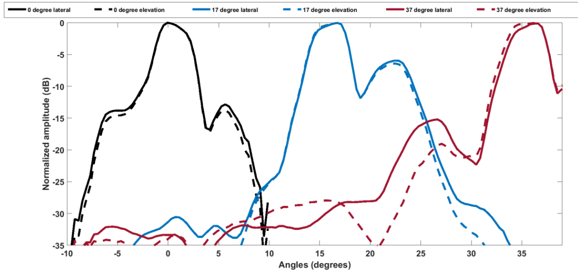
Figure 8.7. Transmit-receive beam profile of the prototype in lateral and elevation directions for three different steering angles ((0°,0°), (17°,17°), and (37°,37°)).
