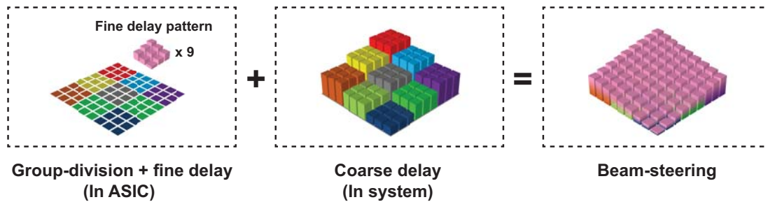
Figure 7.4. The operation principle of micro-beamforming; the height of each bar represents the time delay applied to the signal received by the corresponding element of the array.
