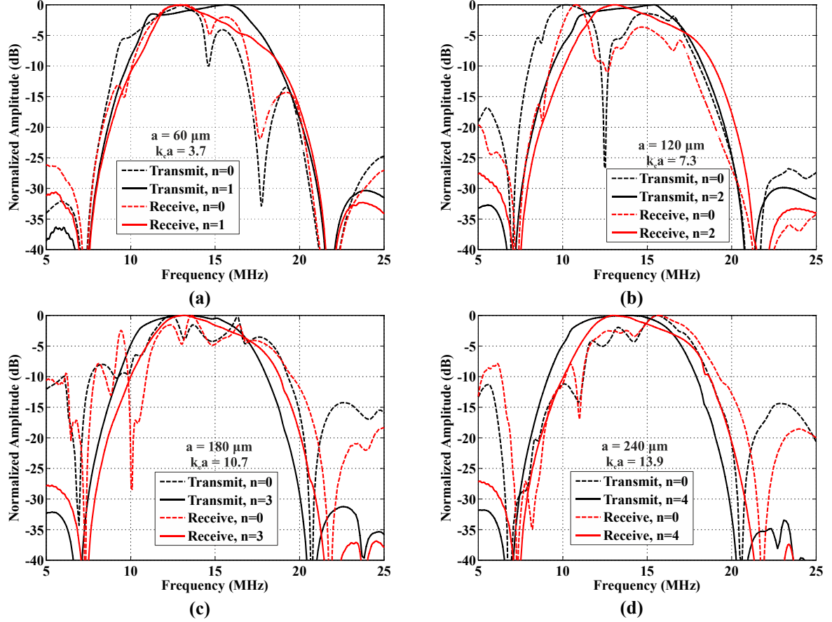
Figure 2.6. Frequency responses in transmit and receive for elements of size, (a) a = 60 \mu\text{m} ( k_c a \cong 3.7 ), (b) a = 120 \mu\text{m} ( k_c a \cong 7.3 ), (c) a = 180 \mu\text{m} ( k_c a \cong 10.7 ), and (d) a = 240 \mu\text{m} ( k_c a \cong 13.9 ). Plots for both the nonsubdiced ( n = 0 ) and the optimally subdiced ( n \neq 0 ) case are given.
