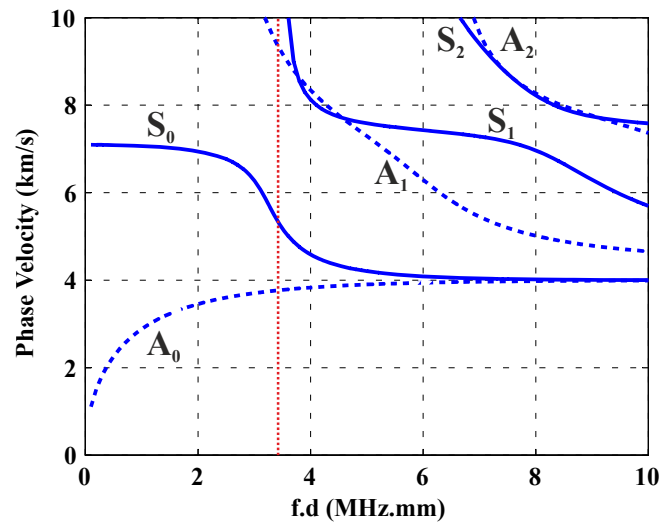
Figure 4.4. Dispersions curves of free Lamb waves for silicon material, calculated with the dispersion toolkit in PZFlex.
