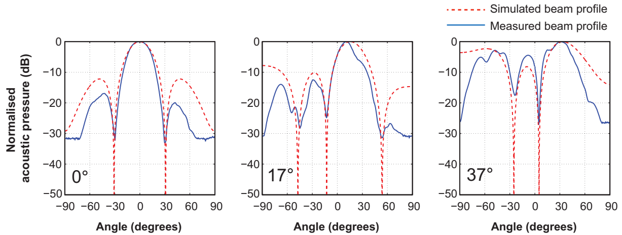
Figure 7.15. Measured and simulated beam profile of a 3 \times 3 micro-beamformed sub-array excited by a 20-cycle sinusoidal pulse at 5 MHz, for steering angles of 0^\circ , 17^\circ and 37^\circ .
