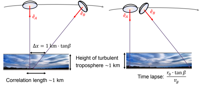
Fig. 1. Sketch of the different acquisition geometries under investigation. The atmospheric boundary layer, which has a height between 1 – 2 km, is highly correlated for the two squints (lines of sight). (Left) Simultaneous and (right) quasi-simultaneous acquisitions by using the bistatic and monostatic modes, respectively.
