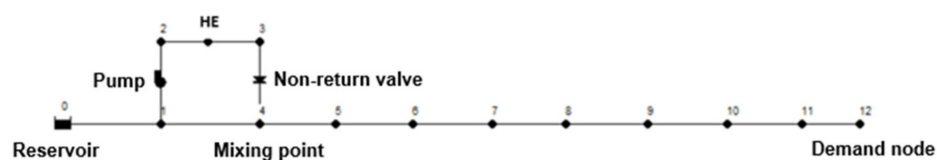
Figure 2. Sanquin full-scale model in EPANET. 0—inlet point/reservoir, 1—4 bypass to the Heat exchanger, HE—heat exchanger, 4—mixing point, 5–11 fictitious points, the mixing point (4), and demand node (12) used to assign measured diurnal flow. The distance between the fictitious points is 500 m, except for the distance between fictitious points 11 and 12, which is 350 m.
