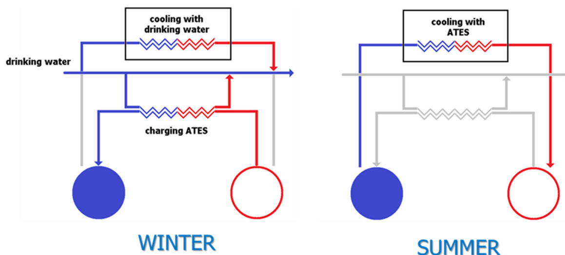
Figure 1. Cold drinking water in wintertime ( left ) is directly utilized in winter periods for places with extensive cooling requirements or is used for charging an aquifer thermal energy storage system (ATES) to provide space cooling in upcoming summer periods ( right ).
