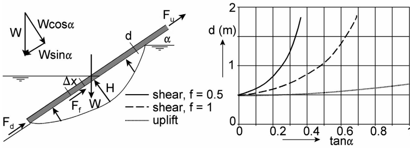
Figure 5-8 Stability of impervious layer on slope
