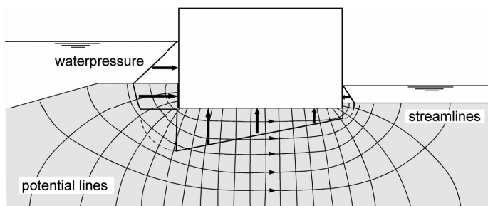
Figure 5-4 Groundwater flow under a caisson
