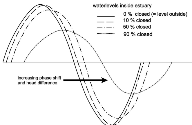
Figure B-5 Waterlevel variations for various phases of the closure
