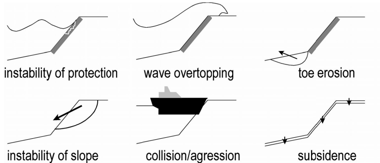
Figure 1-15 Failure mechanisms
