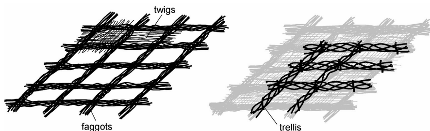
Figure 11-7 Fascine mattress
