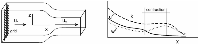
Figure 2-8 Turbulence in wind tunnel contraction (from: Reynolds, 1977)
