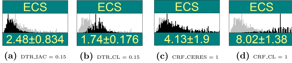
Figure 7: Conditional distribution of ECS given the same observations, measured on different measurement systems, using the static NPNB model from 2050.
