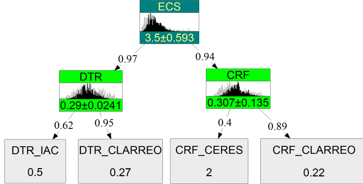
Figure 9: Conditioning the enhanced measuring system variables at their expected values followed by conditioning the current measuring systems' variables at their expected values in the static 2050 model.
