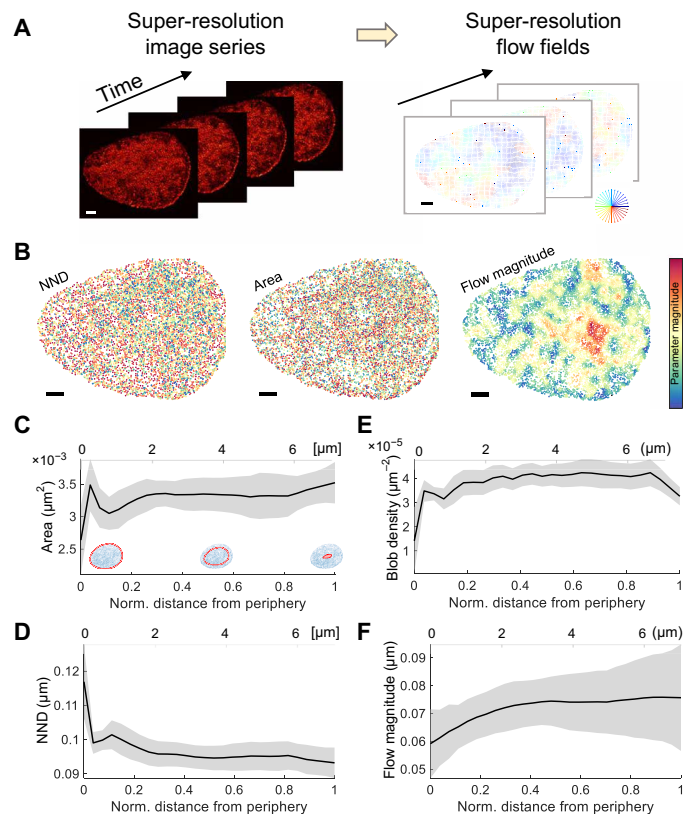
Fig. 4. Structural and dynamics blob characteristics dependent on the proximity to the nuclear periphery. (A) A time series of super-resolution images (left) is subject to optical flow (right). (B) Blobs of a representative nucleus (see movie S1) are labeled by their NND (left), area (middle), and flow magnitude (right). Colors denote the corresponding parameter magnitude. (C) The average blob area, (D) NND, (E) density, and (F) flow magnitude are shown versus the normalized distance from the nuclear periphery (lower x axis; 0 is on the periphery and 1 is at the center of the nucleus) and versus the absolute distance (upper x axis). Line and shaded area denote the means \pm SE from 322 super-resolved images of two cells. Scale bar, (A) and (B): 3 \mu m.
