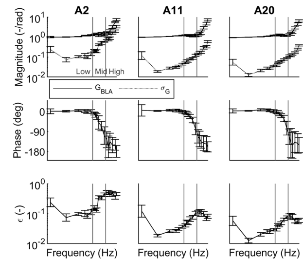
Figure 3: Mean and standard deviation over all participants of the magnitude of G_{BLA} (upper row, solid) and square root of the sample variance ( \sigma_G ) (upper row, dotted), both normalized for the gravitation force, phase of G_{BLA} (middle row) and relative variability \epsilon (bottom row) for the A2, A11 and A20 condition. The three areas between the two vertical grey lines represent the three frequency groups.
