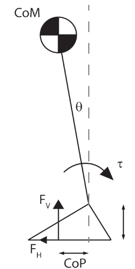
Figure 1: Free body diagram of an inverted pendulum. The joint torque ( \tau ) is calculated by summing the vertical ground reaction forces ( F_v ) multiplied by the centre of pressure (CoP) and the horizontal ground reaction forces ( F_H ) multiplied by the height of the joint ( h ).
