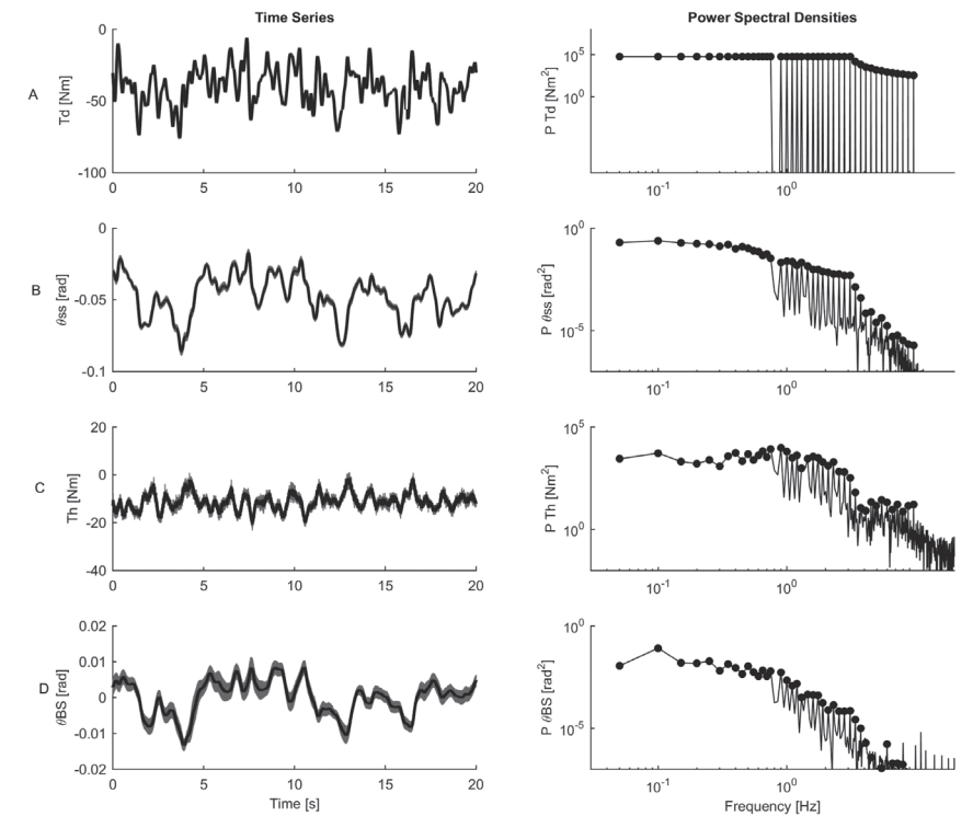
Figure 2: (Left) Time series of a typical subject for the trial with medium support surface (SS) stiffness and medium SS rotation amplitude, in which the disturbance torque ( T_d ), SS rotation amplitude ( \theta_{SS} ), corrective ankle torque ( T_h ) and body sway angle ( \theta_{BS} ) are shown. The mean of the time series is displayed in black and the standard errors in grey. For display purposes, signals were filtered with a phase preserving fourth order low pass digital Butterworth filter with cut-off frequency of 20 Hz. (Right) The associated power spectral densities are shown with the excited frequencies as dots.
