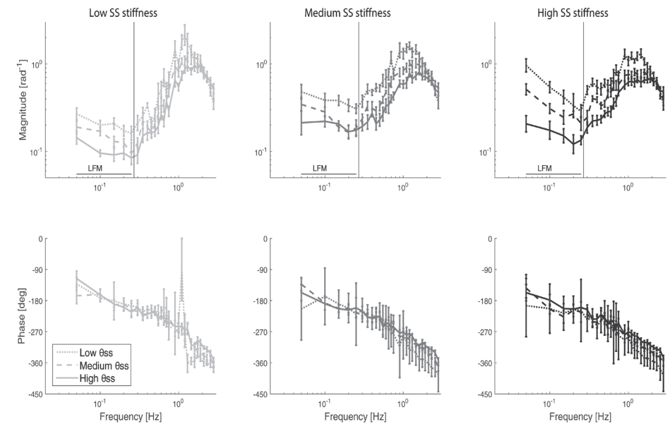
Figure 4: Mean and standard error of the Frequency Response Functions (FRF) of the sensitivity function ( ^{SS}S_{Tn} ), averaged over all subjects, normalized by gravitational stiffness. For each level of support surface (SS) stiffness (low, medium and high K_{SS} ), the effect of SS rotation amplitude (low, medium and high \theta_{SS} ) on the FRF is shown. The vertical line indicates the lower frequency window over which statistical analysis is performed. The lower frequency magnitude (LFM) was calculated by averaging the magnitude of the five lowest frequency magnitudes from 0.05-0.25 Hz.
