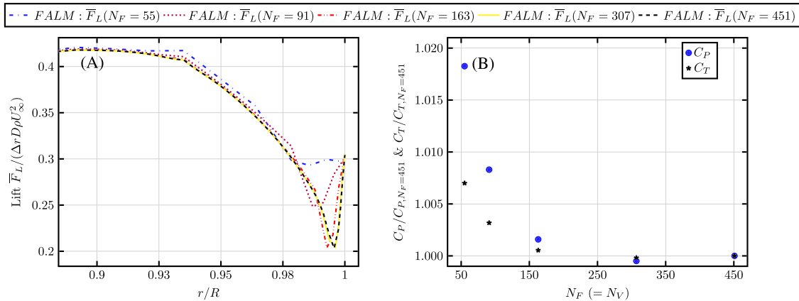
FIGURE C2 Convergence of the filtered actuator line model (FALM) results ( \epsilon/D = 0.11 ) for the NREL 5-MW turbine with increasing number of actuator points ( N_F = N_V ) shown for the lift force per unit length in the outer region of the blade (A) and the aerodynamic thrust and power coefficients of the rotor normalized with their respective values obtained for N_F = 451 (B).
