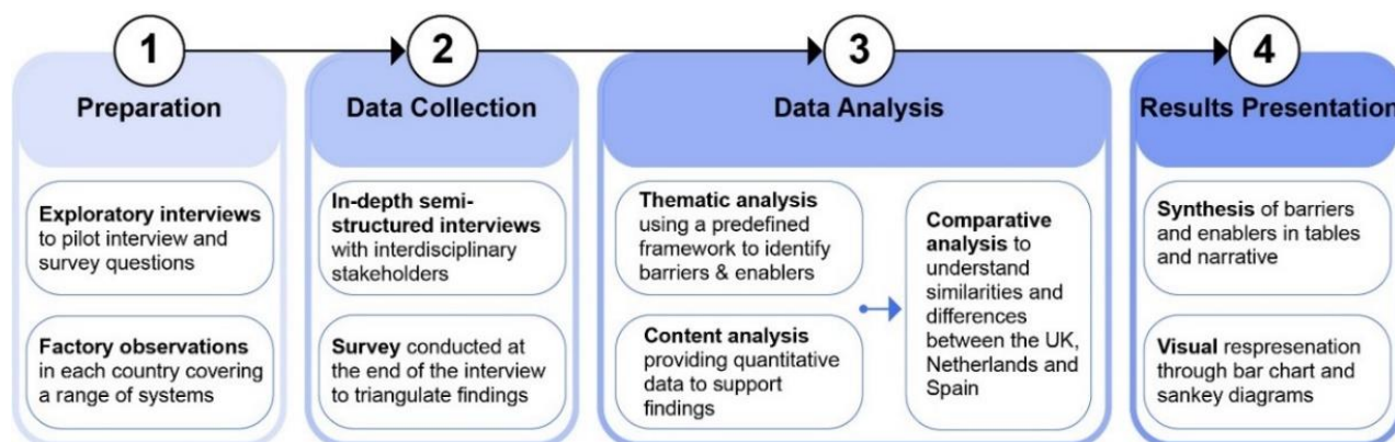
Figure 3. Methodology overview
