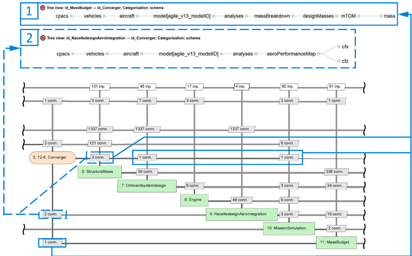
Fig. 19. VISTOMS generated XDSM showing details of the DOE system convergence loop.
