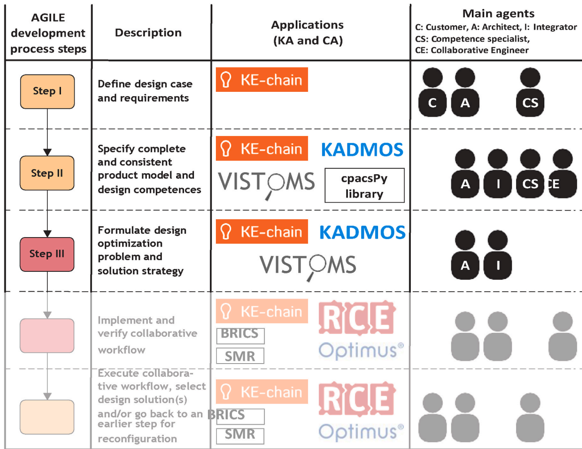
Fig. 4. Five-step AGILE development process with the first three steps highlighted as they are enabled by the KA applications. The final two steps are mainly involving CA applications.
