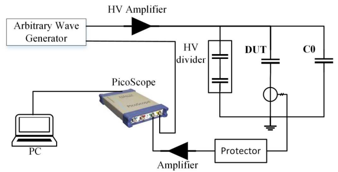
Fig. 1 Experiment setup for (a) flashover test and (b) PD test
