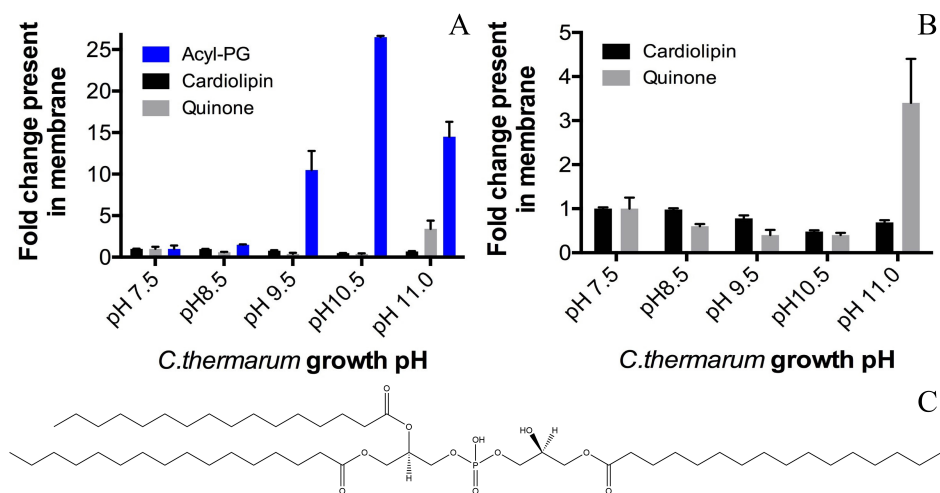
Figure 3.1: Fold changes of Acyl-PG ( A ) and cardiolipin and quinone ( A and B ) abundances relative to pH 7.5. Natta projection ( C ) of an all C 16:0 acyl-PG: 1,2-dipentadecanoyl- sn -glycero-3-phospho-(3'-pentadecanoyl)-1'- sn -glycerol (also used in molecular dynamics simulations in this study).
