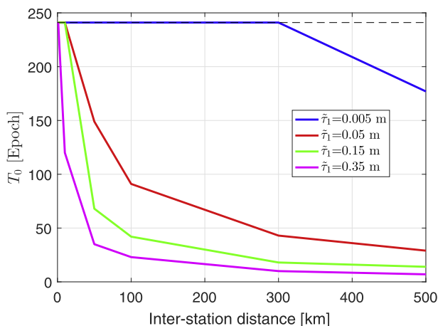
Fig. 9. Minimal number of epochs that is needed to turn the mean RMSE differences of the estimated user coordinates \Delta\text{RMSE}(\hat{\Delta}\hat{x}_u) (43) from positive to negative values. The ambiguity-float network corrections are used for the processing with user ambiguities assumed to be fixed. The T_0 is set to be 241 epochs (see the black dashed line), if it exceeds the 2 h processing interval of 240 epochs.
