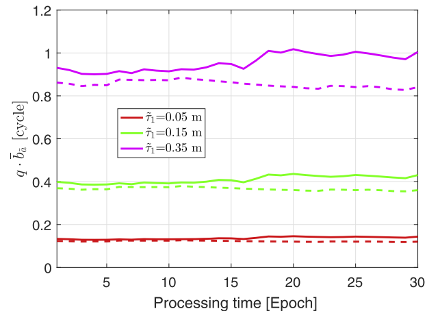
Fig. 6. The mean biases \bar{b}_a of ambiguities under Scenario B (37) for networks with inter-station distances of 50 km (solid lines) and 500 km (dashed lines) that are multiplied by factors q of 10 and 1, respectively.
