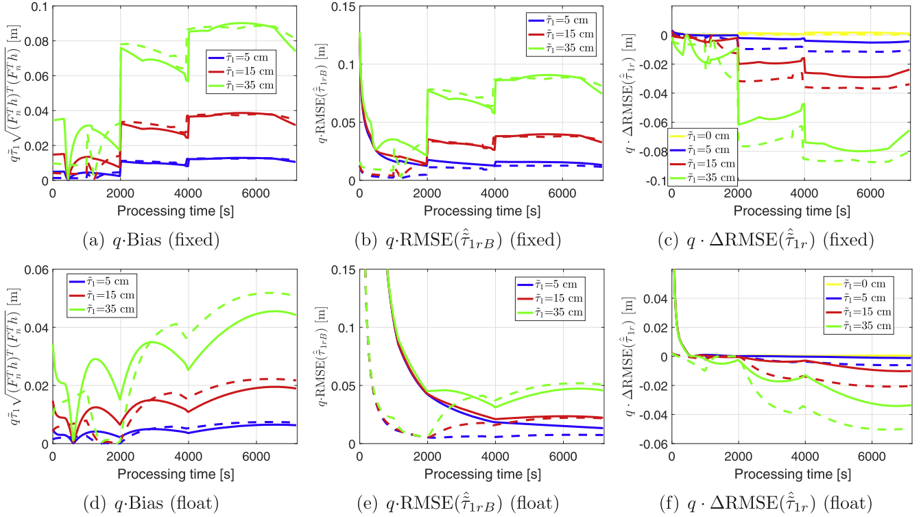
Fig. 5. The bias term \tilde{\tau}_1 \sqrt{(F_n^T h)^T (F_n^T h)} (9) multiplied by factor q for relative ZTDs between stations 1 and 2 with (a) fixed and (d) float ambiguities, the corresponding RMSEs of \hat{\tau}_{1r} under Scenario B (9) and RMSE differences (34) multiplied by q in (b, c) ambiguity-fixed and (e, f) -float cases. The solid and dashed lines represent the cases using the networks located in west of Australia with inter-station distances of 50 and 500 km with factors q of 10 and 1, respectively. The data is processed for the first two hours on June 10, 2017.
