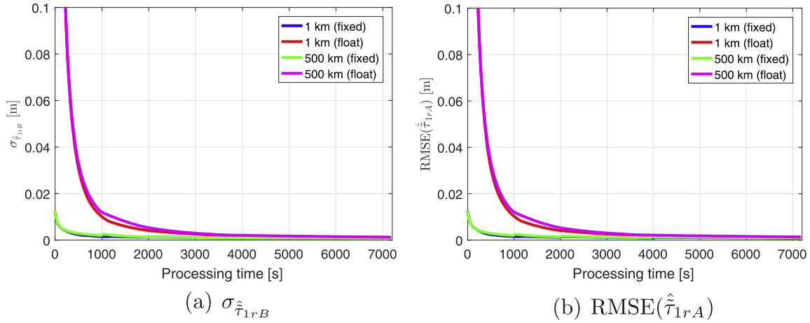
Fig. 4. (a) The formal standard deviations of the relative ZTDs between receivers 1 and 2 under Scenario B and (b) their RMSEs under Scenario A (9) using the networks located in west of Australia with inter-station distances of 1 km and 500 km. The data is processed for the first two hours on June 10, 2017.
