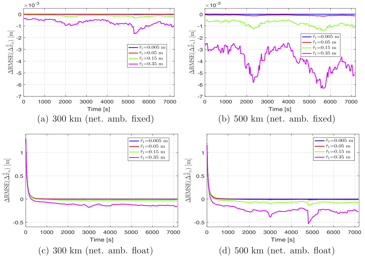
Fig. 8. Mean RMSE differences (42) of the estimated user coordinates for networks with inter-station distances of 300 km (left) and 500 km (right) where ambiguity-fixed (top) and -float (bottom) network-corrections are applied. The user ambiguities are assumed to be resolved. We note that in (c) the blue line is almost overwritten by the red line. (For interpretation of the references to color in this figure legend, the reader is referred to the web version of this article.)
