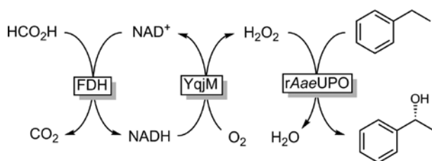
Scheme 1: Proposed in situ H 2 O 2 generation system to promote the stereoselective hydroxylation of ethyl benzene to ( R )-1-phenyl ethanol using the recombinant peroxygenase from A. aegerita (rAaeUPO). In situ H 2 O 2 generation is achieved by reductive activation of O 2 through a cascade of FDH-catalysed oxidation of formic acid and concomitant reduction of nicotinamide adenine dinucleotide (NAD + ) to its reduced form (NADH). The latter is reoxidised by the old yellow enzyme homologue from B. subtilis (YqjM) to reduce O 2 to H 2 O 2 .
