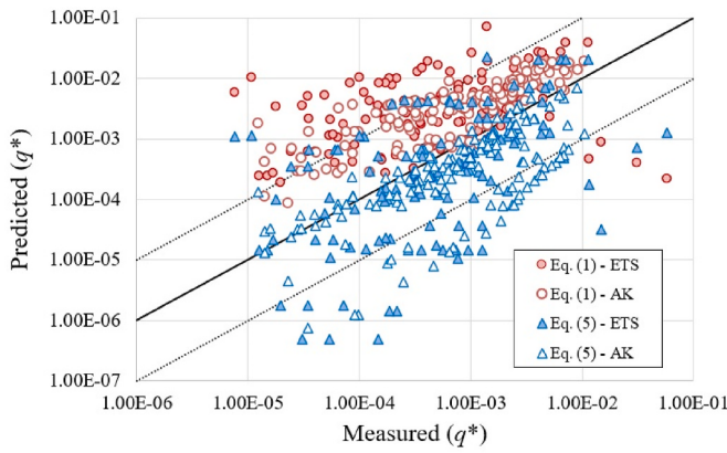
Fig. 4. Predicted vs measured mean wave overtopping rate at rubble mound seawalls using Eq. 1, Owen (1980) and Eq. 5, EurOtop (2018) formulae.
