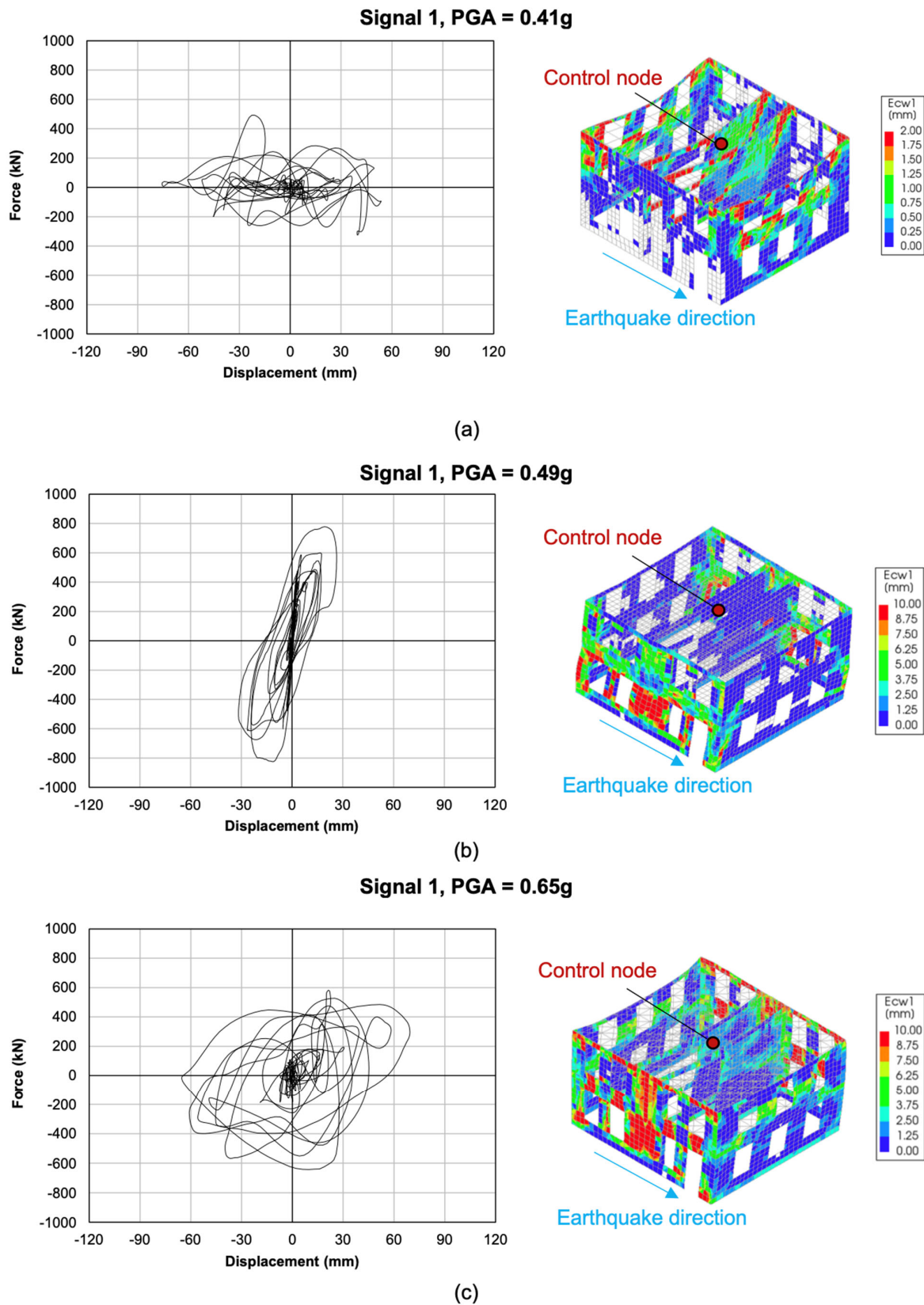
Figure 13. Base shear vs. top roof displacement response and damage level in terms of the principal crack opening (E cw1 ) for the three configurations: B2-AB (a), B2-RC (b), and B2-PP (c) at a near-collapse state.
