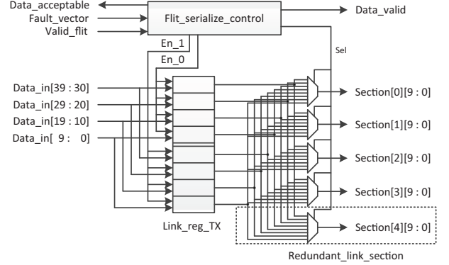
Fig. 2. Flit serialization unit - TX.
