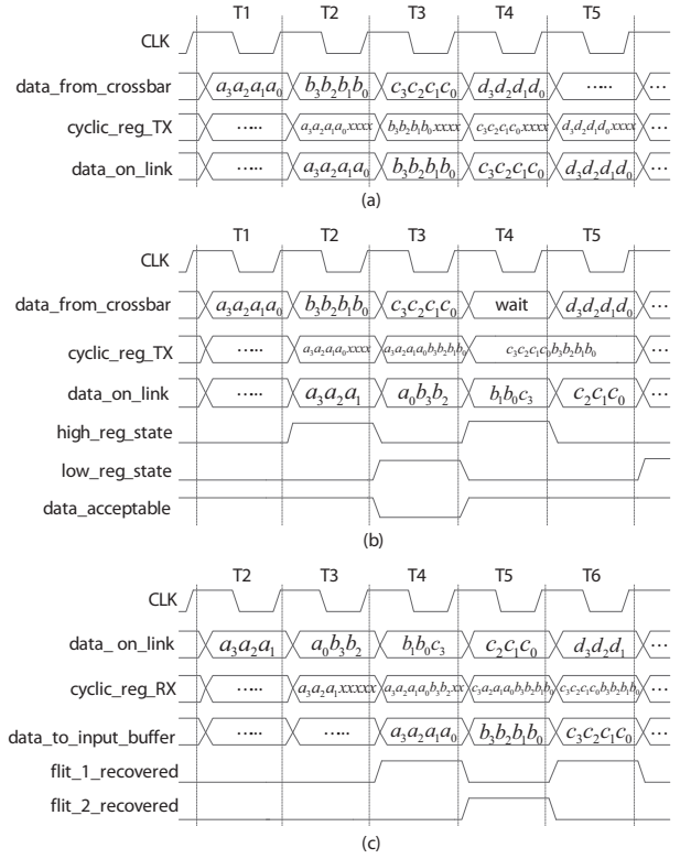
Fig. 4. Timing diagram of proposed mechanism (a) Timing diagram for a fault-free link; (b) Transmitter side when one section contains faulty wires; (c) Receiver side when one section contains faulty wires.
