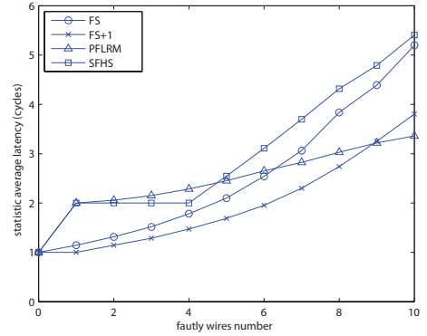
Fig. 5. Average flit transmission latency of different partially faulty link utilization strategies. The link is divided into 8 sections for FS and SFHS.
