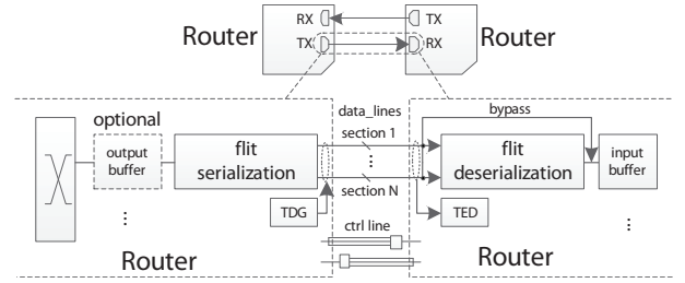
Fig. 1. Proposed fault-tolerant link architecture.
