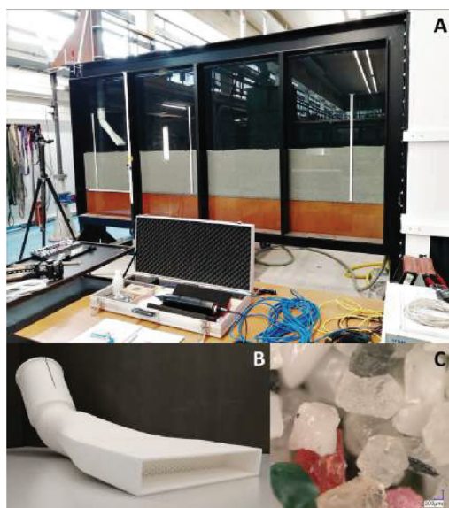
Figure 2: Experimental setup: (a), the 2D and 3D-printed water jet (b), and sediment (c).
