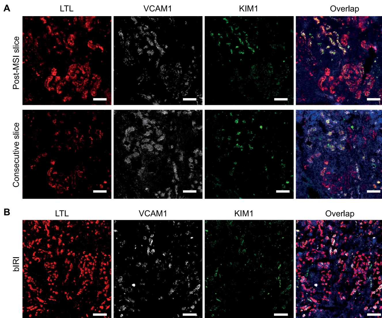
Extended Data Fig. 6 | Immunofluorescence staining on mouse IRI kidneys. a, Validation of immunofluorescence staining of LTL, VCAM1 and KIM1 on the measured area of post-MSI slice compared to consecutive slice without MALDI matrix. Scale bar = 100 \mu\text{m} . b, Immunofluorescence staining of LTL, VCAM1 and KIM1 on bIRI kidney, same as the image shown in Fig. 4b. Scale bar = 200 \mu\text{m} .
