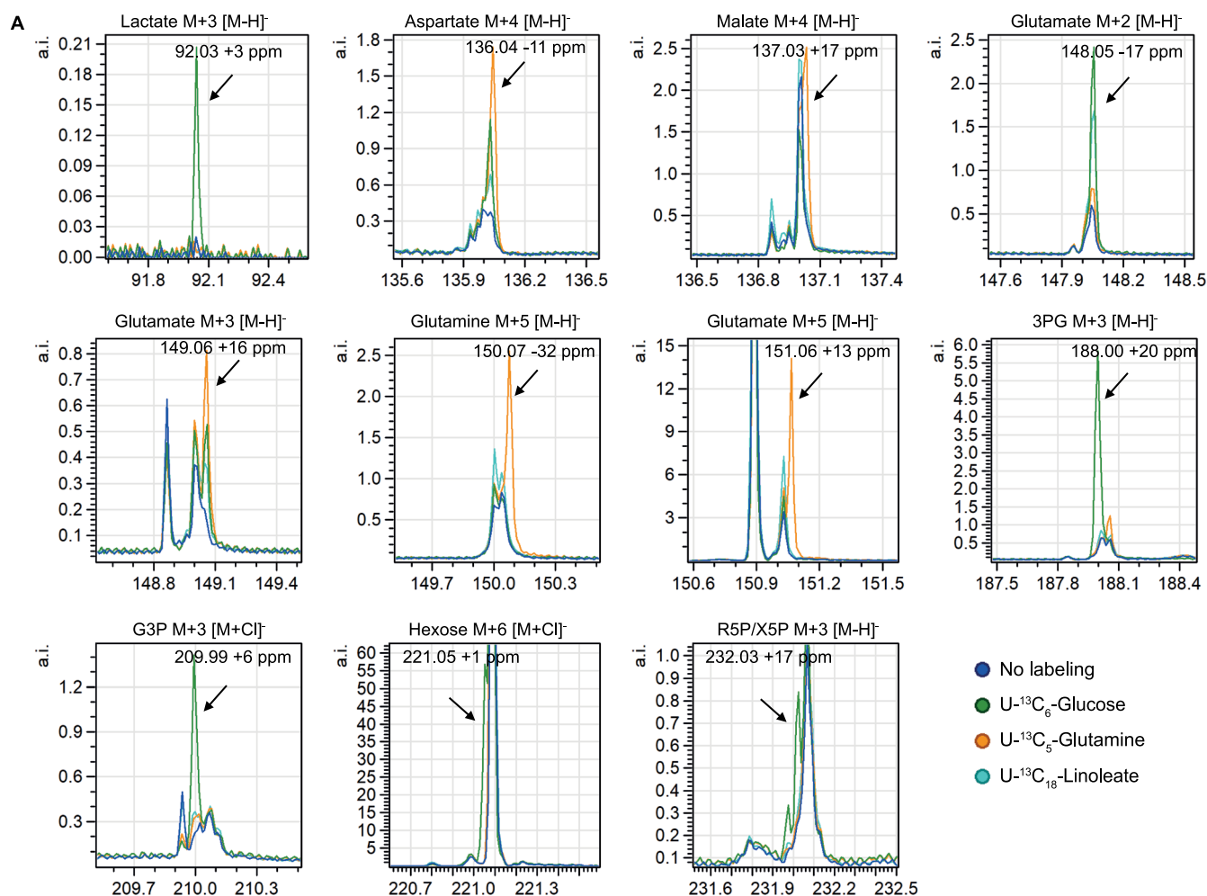
Extended Data Fig. 2 | Mass spectrum of measured 13 C-labeled Metabolites. Mass spectra obtained from 13 C-labeled- and control samples measured by MALDI-MSI at 5×5 μm 2 pixel size. Graphs show presence of various 13 C-labeled metabolites.
