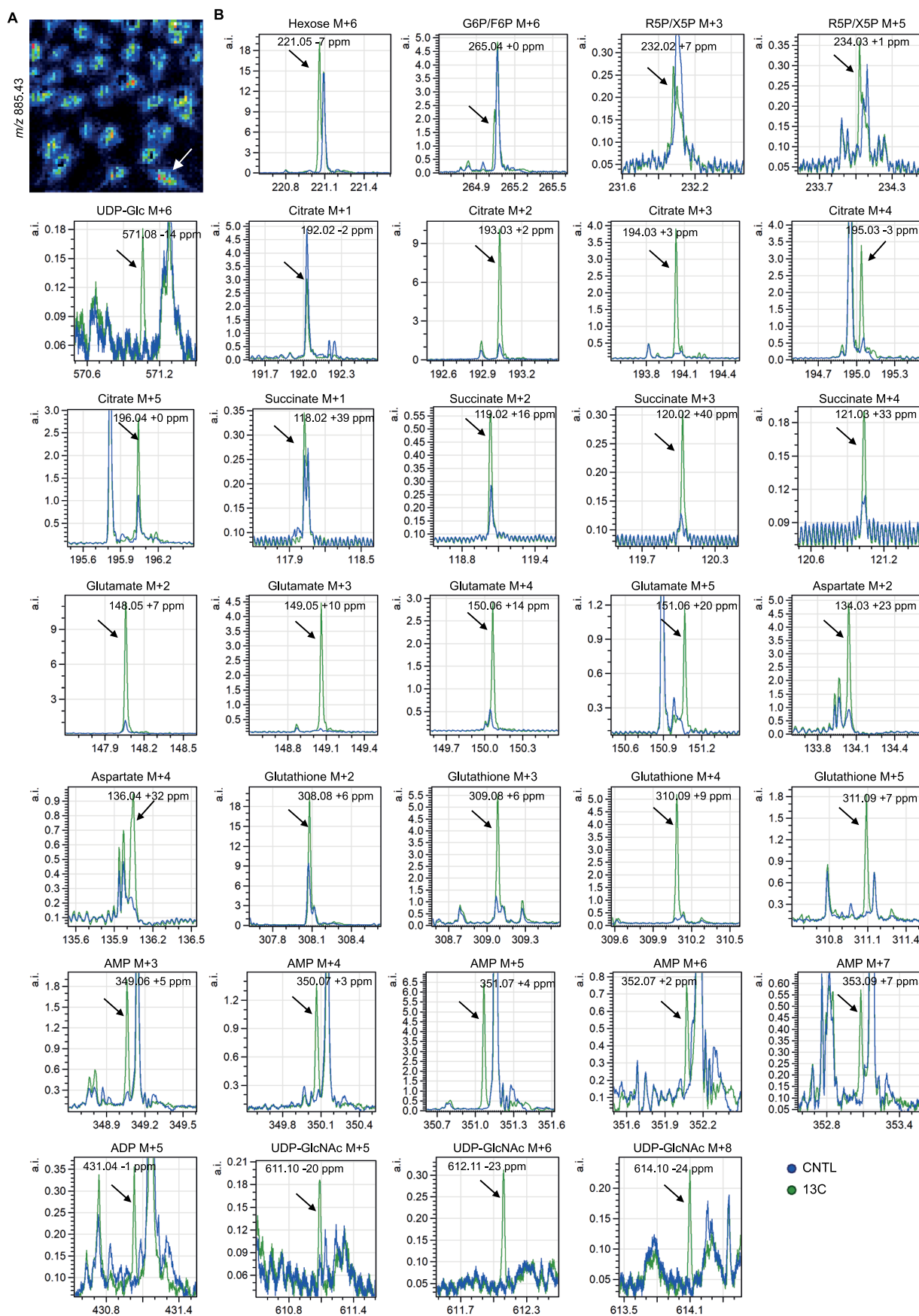
Extended Data Fig. 8 | High spatial resolution MALDI-MSI measurement on cultured endothelial cell. a , MALDI-MSI data from measurements of cultured endothelial cells, which were incubated with U\text{-}^{13}\text{C}_6 -glucose for 24 h. Arrow depicts a single endothelial cell. b , Mass spectra obtained from ^{13}\text{C} -labeled- and control samples measured by MALDI-MSI at 5 \times 5 \mu\text{m}^2 pixel size to show the presence of ^{13}\text{C} -labeled metabolites.
