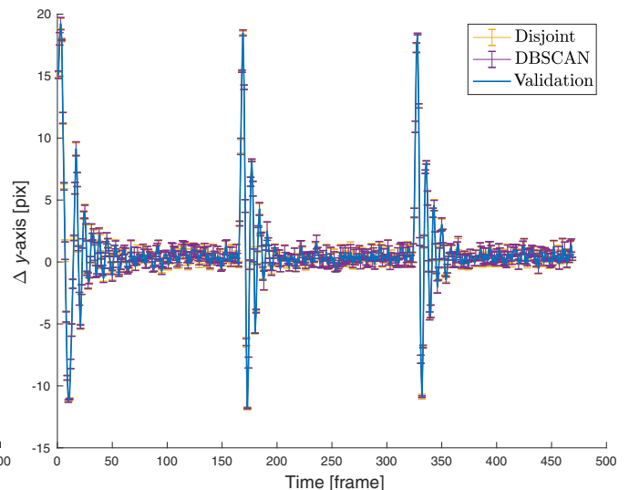
d) Displacement in y of R1 sequence marker ID 7
