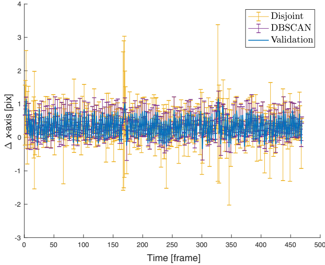
a) Displacement in x of R1 sequence marker ID 2
