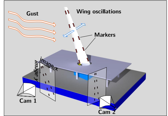
Fig. 2 Experimental setup with the wing facing the wind tunnel, equipped with visual markers.
