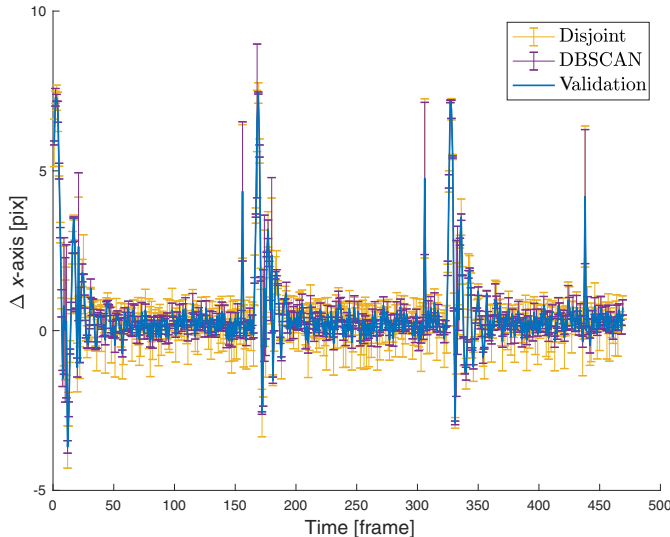
c) Displacement in x of R1 sequence marker ID 7
