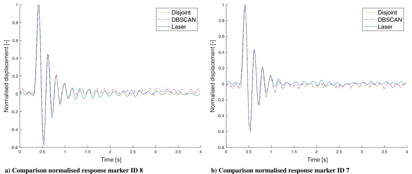
Fig. 22 Comparison of normalized response of the tip deflection for run R1 (laser vs image tracking).
