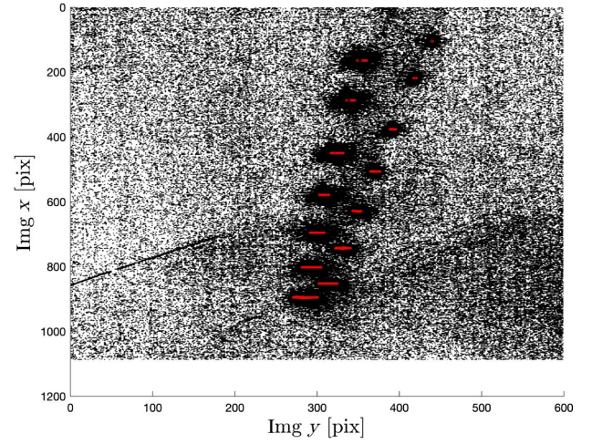
b) Top view global normalisation thresholding
