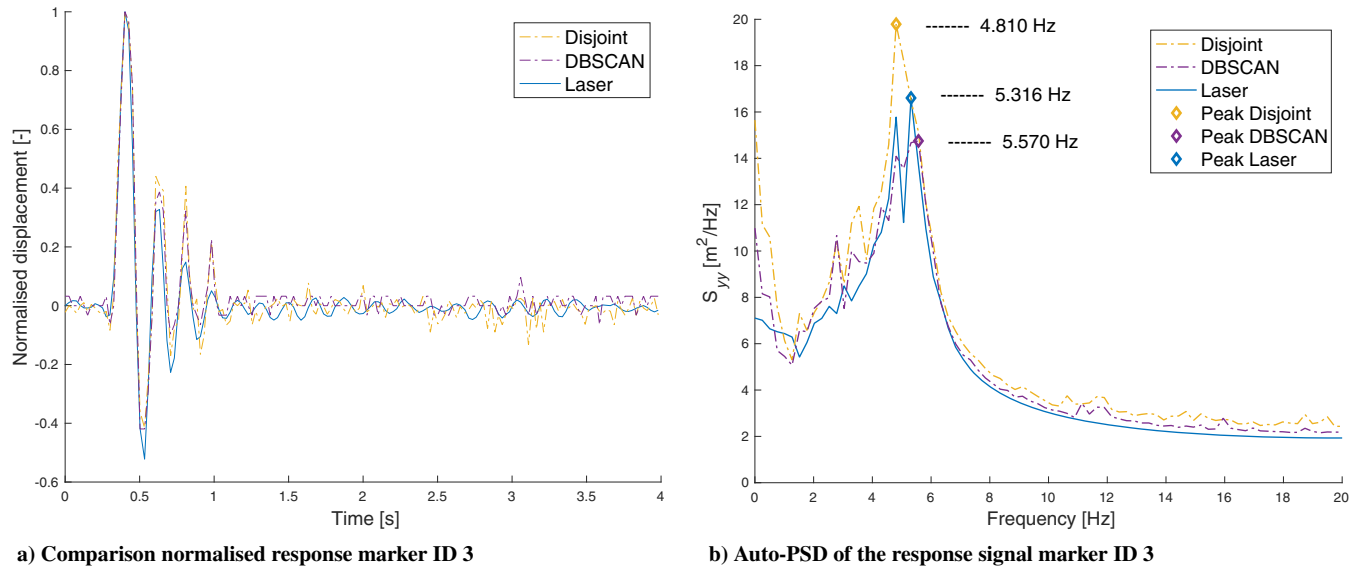
Fig. 24 Comparison of the response and the frequency spectrum of the marker ID 3, run R1 (laser vs image tracking).
